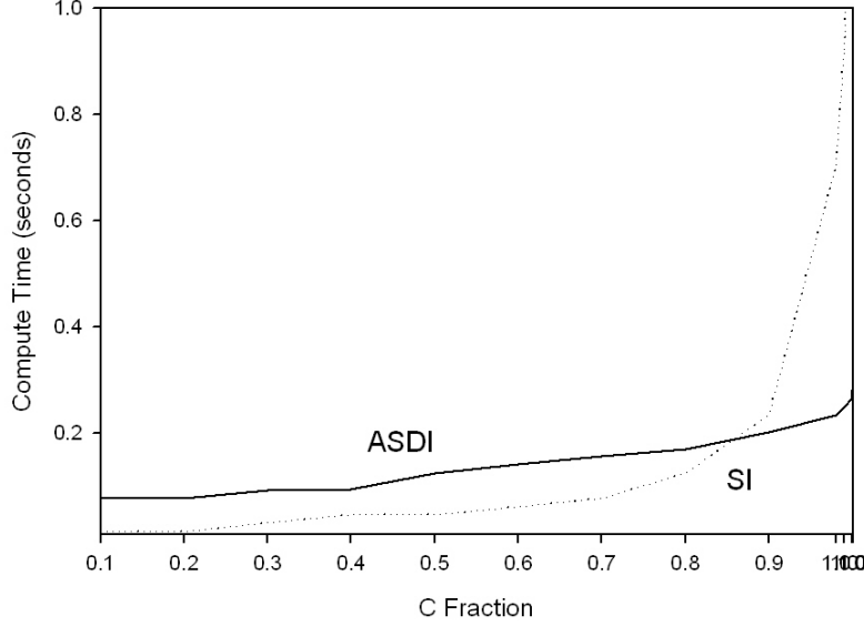
Figure 31 Plot of compute time (seconds) versus scattering ratio. Angular quadrature is DE-8, refinement is 50 ( \sigma\Delta x = 2 \text{ MFPs} ), convergence tolerance is 10^{-6} .
