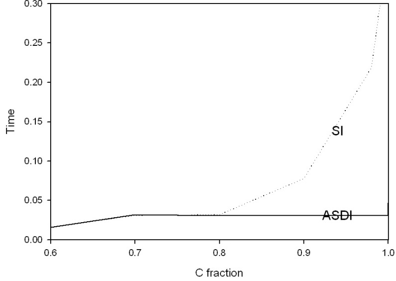
Figure 7 Plot of compute time (seconds) versus scattering ratio. Angular quadrature is DE-8, refinement is 50 ( \sigma\Delta x = 2\text{ MFPs} ), convergence tolerance is 10^{-6} .
