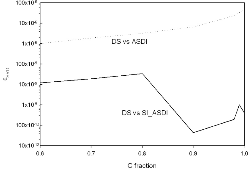
Figure 5: Symmetric Relative Difference \varepsilon_{SRD} between the ASDI solution and the SI
