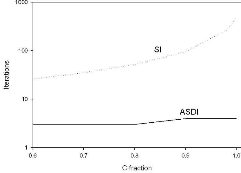
Figure 6 Plot of iteration count versus scattering ratio. Angular quadrature is DE-8, refinement is 50 ( \Delta x = 2 \text{ MFPs} ), convergence tolerance is 10^{-6} .
