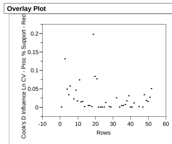
Figure 4.25 – Cook's Distance Overlay Plot for Influential Data Points Support (Reduced) Model (OLS)
