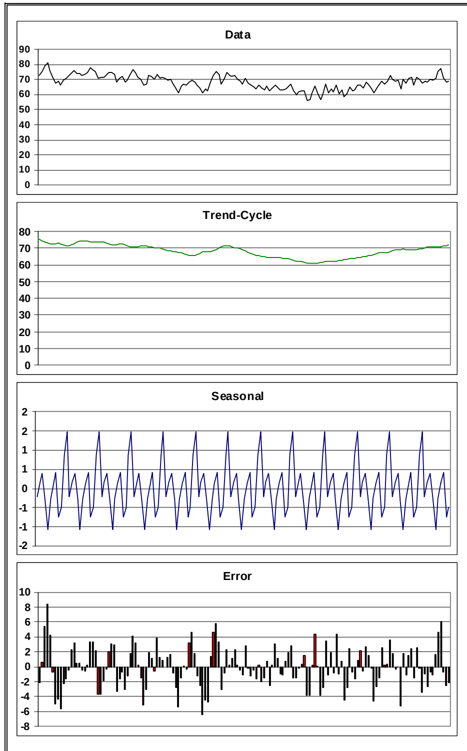
Figure 3. C-5 Galaxy Classical Decomposition of the Complete Data Set
