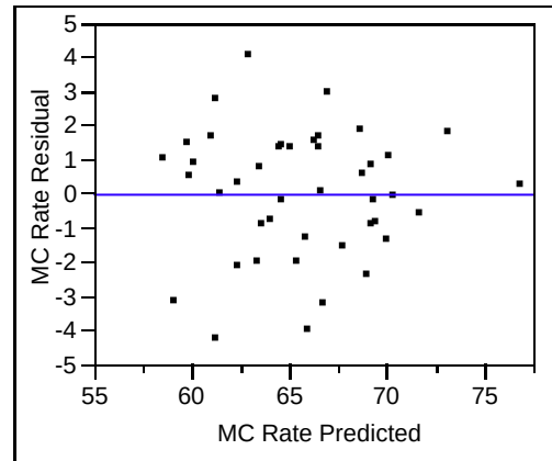
Figure 17. C-5 Galaxy Final Explanatory Model (2) Variance Plot
