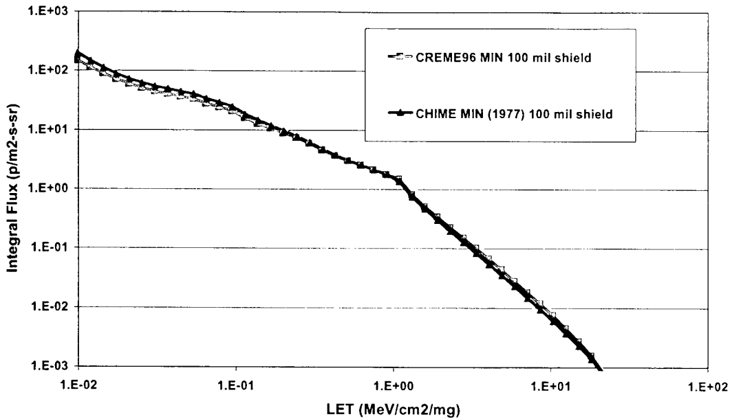
Figure 5. CREME96-CHIME Comparison (Solar Min LET Behind 100 mils Shield)
