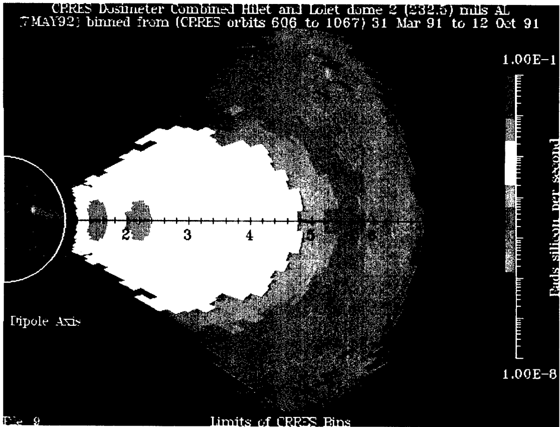
Figure 2. Major Storm-Enhanced Radiation Dose Levels Behind ~1/4 inch Aluminum
