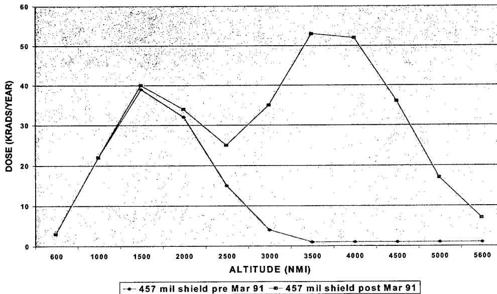
Figure A-3. Radiation Dose Versus Altitude For 3 Shielding Thickness (20° Inclination)
