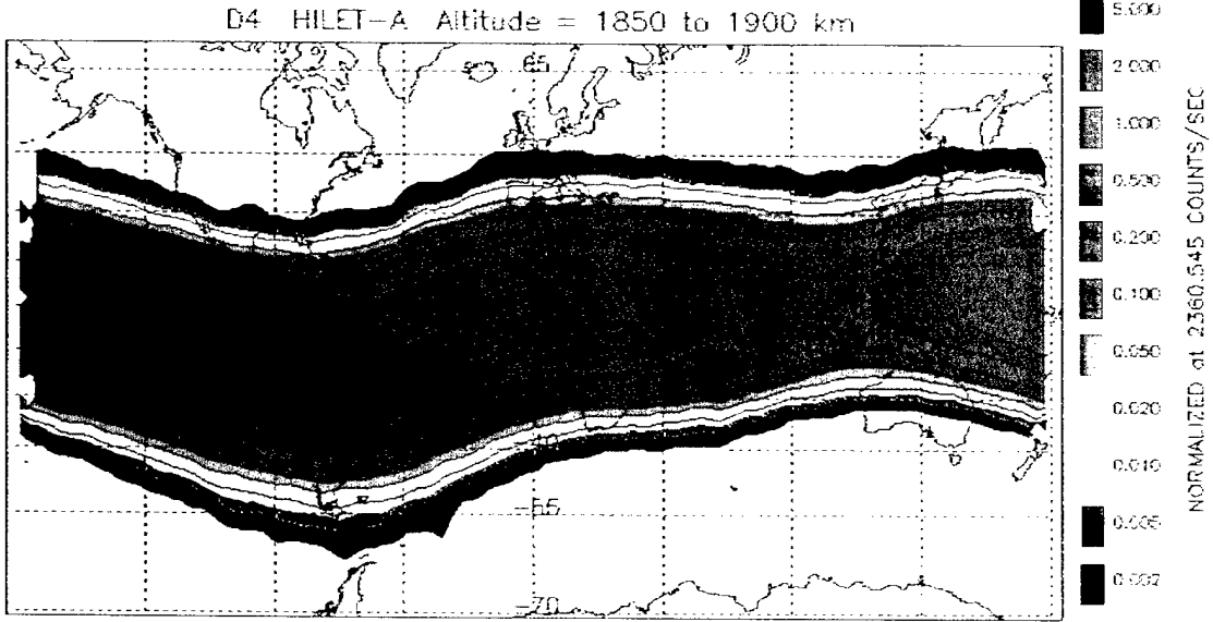
Figure A-4. Relative Probability Of SEUs Due To Protons
