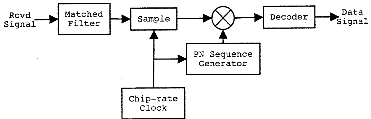
Figure 2: Schematic diagram of a DS-SS receiver.
