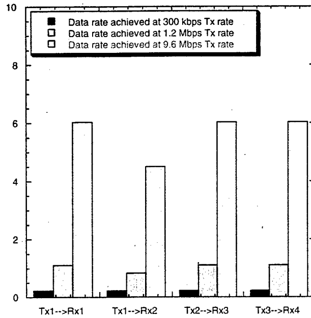
Figure 25: Data rates achieved for various indoor transmission scenarios and transmission rates.
