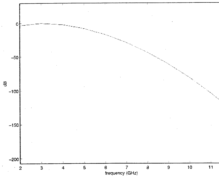
Figure 8: Spectrum of a transmitted Gaussian monocycle.
