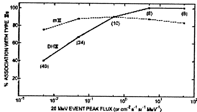
Fig. 1. Percentage association of \sim 20 MeV SEP events with metric type II (dashed line) and DH type II (solid line) bursts as a function of SEP event peak intensity.
