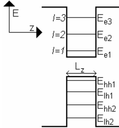
Fig. 2- 17: The quantized energy subbands found in a quantum well structure. This shows the discrete levels formed by the electrons in the conduction band and the heavy-holes and light-holes in the valence band.
