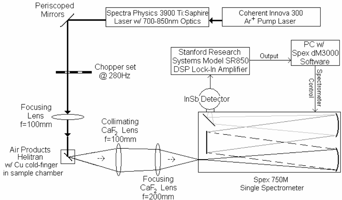
Fig. 3- 3: The table configuration used for this experiment to obtain the photoluminescence from the antimony-based semiconductors.
