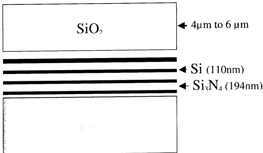
Figure 1. Illustration of an asymmetric PBG cladding waveguide.
