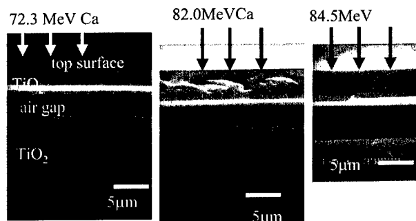
Figures 4. SEM images of the cross section of the sample etched following the (a) 72.3, (b) 82.0, and (c) 84.5 MeV Ca ion irradiation to a dose of 3.0 \times 10^{14} \text{ cm}^{-2} . The ions were irradiated from the top of the image.
