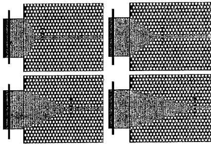
Figure1. Four of the five tapers investigated. The bold and dashed lines show approximately the locations where the input and coupled powers are measured respectively.
