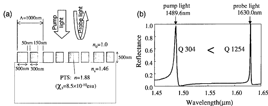
Figure 9. An asymmetric grating wave-guide for a nonlinear optical switch. (a) An asymmetric grating structure with the large second harmonic component. The grating material has third-order susceptibility. (b) Spectral reflectance of the asymmetric grating wave-guide for TE polarized light. There are two resonant peaks with different FWHMs.
