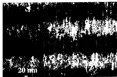
Fig.1. Cross-sectional SEM image of alternating layers with low (36%) and high (59%) porosities.
