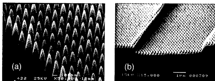
Figure 2. Antireflection structured surfaces on a flat silica surface (a) and a diffraction grating (b). The structure on the flat surface has a period of 250nm and cone height of 750nm (aspect ratio: 3). The structure of the diffraction grating has an aspect ratio of 1.
