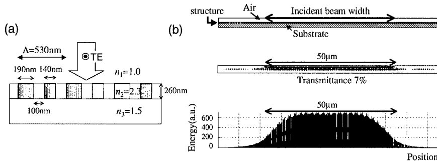
Figure 7. A resonant grating filter with a large second harmonic component (a), and a simulation result of wave localization in the wave-guide layer (b). The incident light beam has a width of 50\mu\text{m} . The bottom figure shows the field energy distribution in the wave-guide layer.
