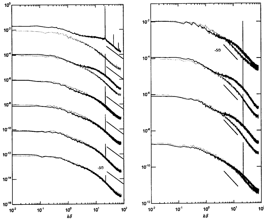
Figure IV.17 u power spectra (baseline is in gray). Left: y/\delta = 0.065 ( y^+ = 60 ), x/\delta = 0.16, 0.65, 1.3, 1.9, 2.6, and 3.5 (top to bottom). Right: x/\delta = 0.65 , y/\delta = 0.032, 0.065, 0.097, and 0.16 (top to bottom) ( y^+ = 30, 60, 90, and 145 ). Successive locations displaced by two decades.
