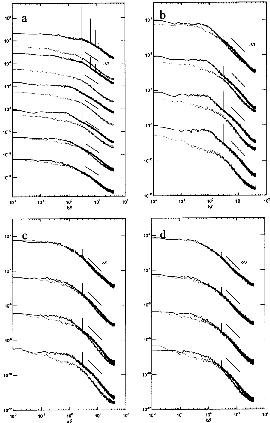
Figure IV.28. u power spectra: a) y/\delta = 0.32 ( y^+ = 85 ), x/\delta = 0.8, 1.5, 3.0, 6.1, 12, and 18 (top to bottom), b) x/\delta = 6.1 , y/\delta = 0.08, 0.16, 0.32, and 0.64 (top to bottom) ( y^+ = 21, 43, 85, and 170 ), c) x/\delta = 12 , y/\delta = 0.08, 0.16, 0.32, and 0.64 (top to bottom) ( y^+ = 21, 43, 85, and 170 ), and d) x/\delta = 18 , y/\delta = 0.08, 0.16, 0.32, and 0.64 (top to bottom) ( y^+ = 21, 43, 85, and 170 ). Baseline in gray, actuated solid line. Successive spectra displaced by two decades.
