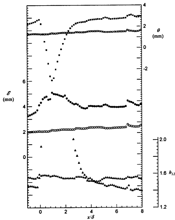
Figure IV.26. Boundary layer evolution, baseline: \delta^* ( \circ ), \theta ( \square ), h_{12} ( \Delta ); actuated: \delta^* ( \bullet ), \theta ( \blacksquare ), h_{12} ( \blacktriangle ).
