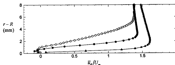
Figure I.7 Cross stream velocity distributions, \theta = 100^\circ : baseline (○), tripped (●), actuated (▲).
