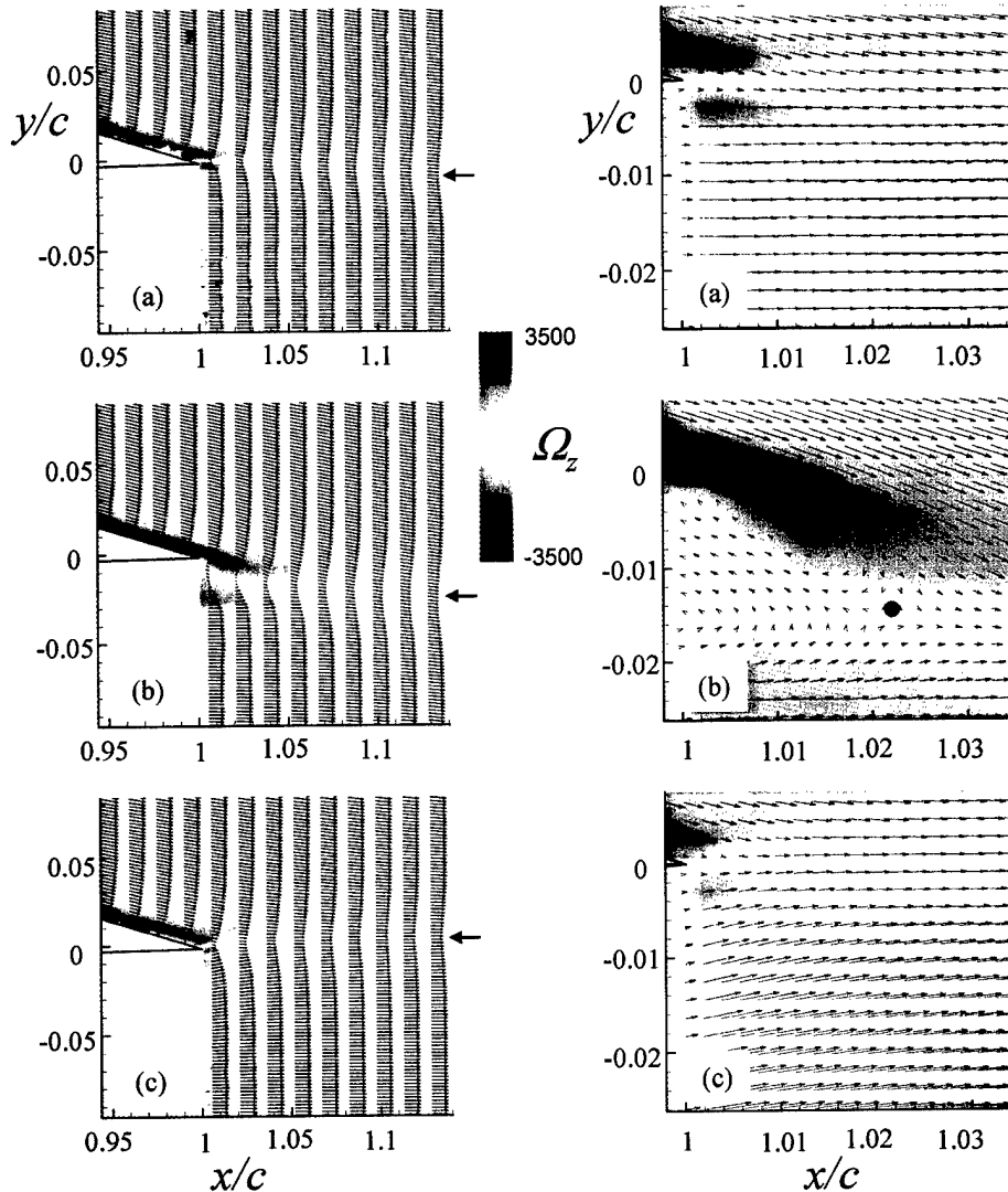
Figure III.9. Global views of superimposed time-averaged maps of spanwise vorticity and cross-stream velocity vectors for the smooth airfoil (a), and with the JIF in the absence (b) and presence (c) of actuation.
