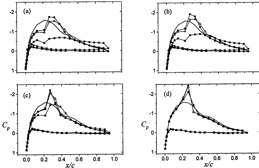
Figure II.14. Pressure distributions around the airfoil at \alpha = 3^\circ and Re_c = 381,000 for (a) f_{act} = 139 Hz, (b) 187 Hz, (c) 362 Hz and (d) 850 Hz. (—) baseline and actuated: ( \bullet ) C_\mu = 1.2 \times 10^{-3} , ( \Delta ) 5.7 \times 10^{-4} , and ( * ) 1.7 \times 10^{-4} .
