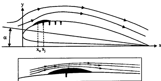
Figure II.4. Airfoil model.
