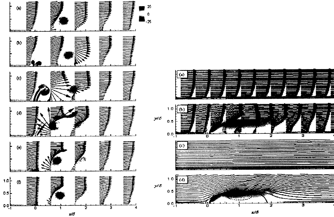
Figure IV.19. Left: Phase-averaged normalized vorticity with superimposed velocity vectors, Re\theta = 700 , St\delta = 0.47 , \bar{U}_y/U_\infty = 1.25 , \delta b = 6.5 : (a) \phi = 0^\circ , (b) 60^\circ , (c) 120^\circ , (d) 180^\circ , (e) 240^\circ , and (f) 300^\circ . Right: Time-averaged normalized vorticity with velocity vectors (a & b) and streamlines (c & d) for baseline (a, c) and actuated (b, d).
