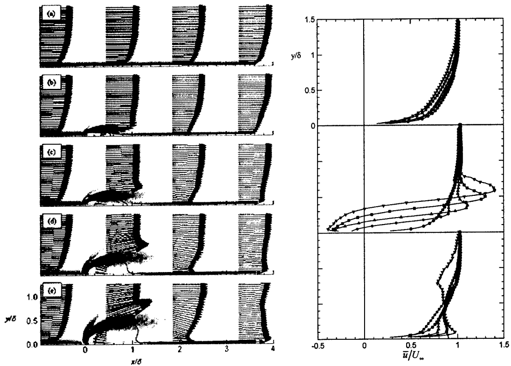
Figure IV.3. Left: Normalized spanwise vorticity, and velocity, Re\theta = 520 , St\delta = 21 , \delta^*b = 73 : (a) baseline, (b) \bar{U}_j/U_\infty = 3.0 , (c) 4.0, (d) 5.0, and (e) 6.0. \psi = 0 is superimposed, and Right: Mean velocity: baseline (○), \bar{U}_j/U_\infty = 3.0 (●), 4.0 (▲), 5.0 (■), and 6.0 (▼). x/\delta = -0.5, 0.5, \text{ and } 3.0 (from top to bottom).
