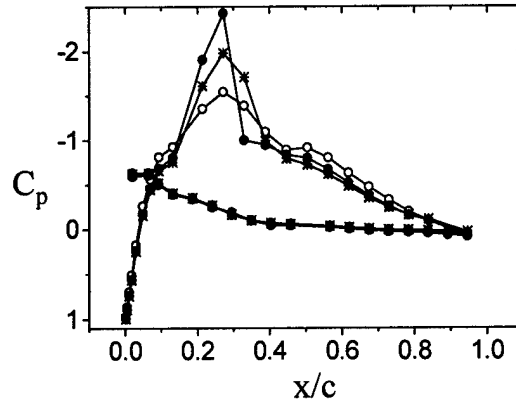
Figure II.9. Pressure distribution around the airfoil at \alpha = 1^\circ . ( \circ ) baseline, ( \bullet ) upstream jet is on and ( * ) downstream jet is on.
