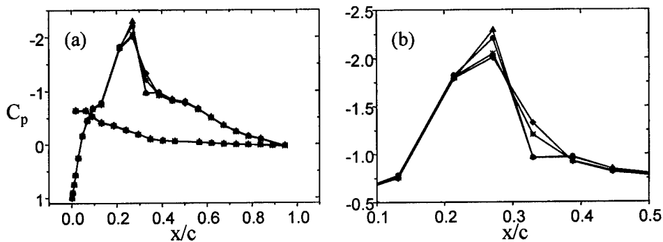
Figure II.12. Pressure distribution around the airfoil at \alpha = 1^\circ . Global distribution (a) and detailed distribution (b). ( \bullet ) C_\mu = 1.9 \cdot 10^{-3} , ( \blacktriangle ) 5.4 \cdot 10^{-4} , ( \star ) 3.1 \cdot 10^{-5} and ( \blacklozenge ) 1.8 \cdot 10^{-5} .
