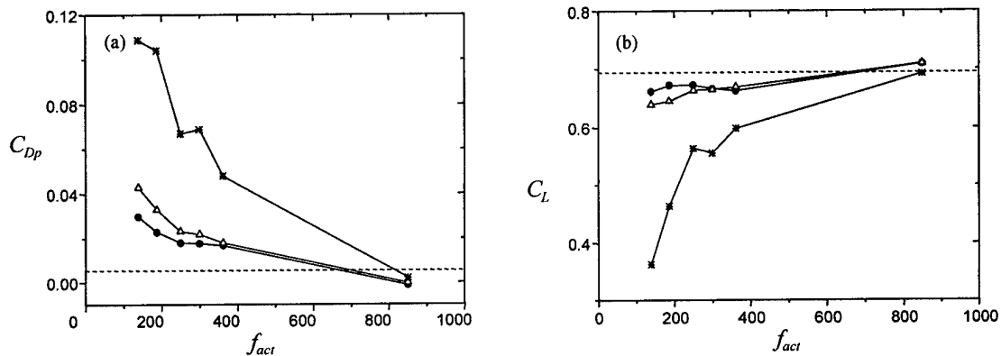
Figure II.16. Pressure drag coefficient (a) and lift coefficient (b) as a function of the actuation frequency. ( \bullet ) C_\mu = 1.2 \cdot 10^{-3} , ( \Delta ) 5.7 \cdot 10^{-4} , and ( * ) 1.7 \cdot 10^{-4} , Re_c = 381,000 . The baseline is represented by the dashed line.
