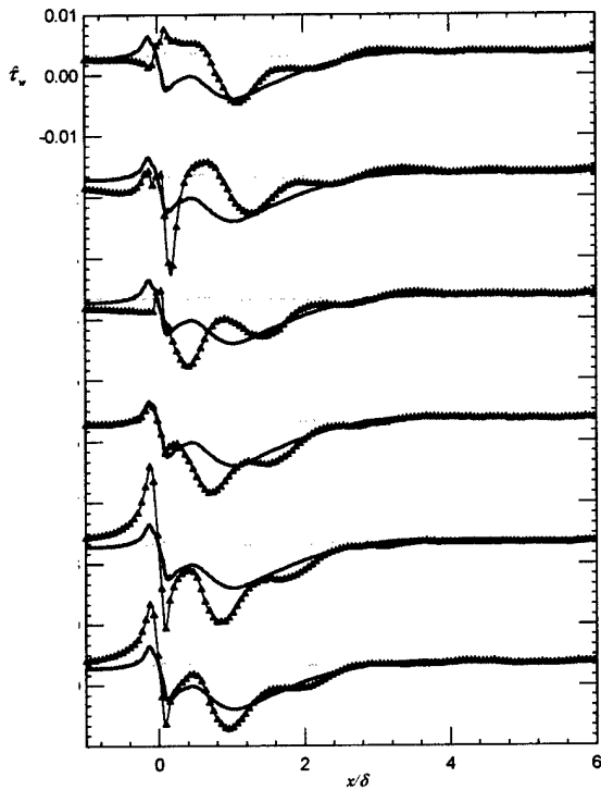
Figure IV.25. Normalized wall shear stress, \phi = 0^\circ, 60^\circ, 120^\circ, 180^\circ, 240^\circ, and 300^\circ (from top to bottom, successive phases separated by 0.02 ): (baseline-gray line; time-averaged actuated-black solid line, phase-averaged \Delta ).
