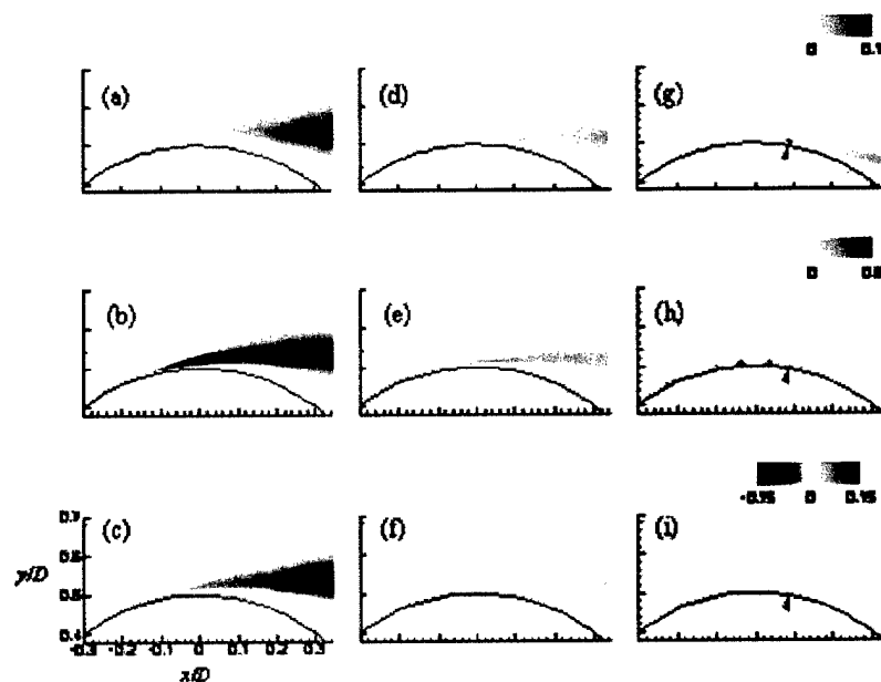
Figure I.8 Normalized Reynolds Stresses: \overline{u'_i u'_i} / U_\infty^2 (a, d, g), \overline{u'_\theta u'_\theta} / U_\infty^2 (b, e, h), \overline{u'_i u'_\theta} / U_\infty^2 (c, f, i); baseline (a, b, c), tripped (d, e, f), actuated (g, h, i).
