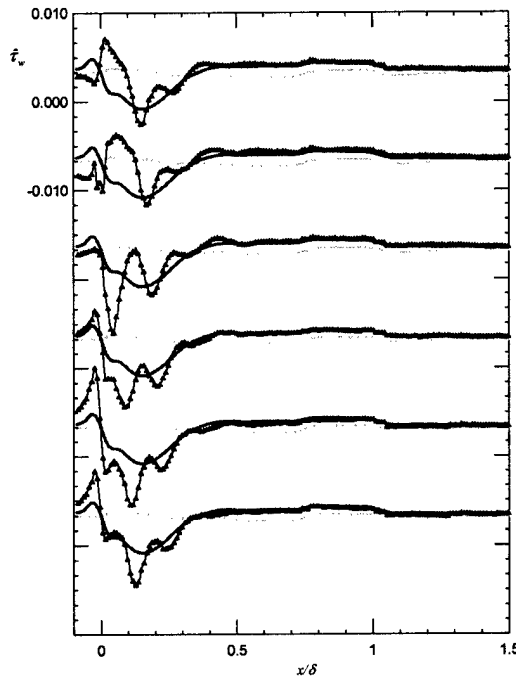
Figure IV.13. Normalized wall shear stress: ( \Delta ) phase-averaged, from top to bottom, \phi = 0^\circ, 60^\circ, 120^\circ, 180^\circ, 240^\circ, and 300^\circ ; — baseline; - - - actuated. Successive phases separated by 0.01
