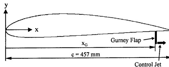
Figure III.2. Airfoil model
