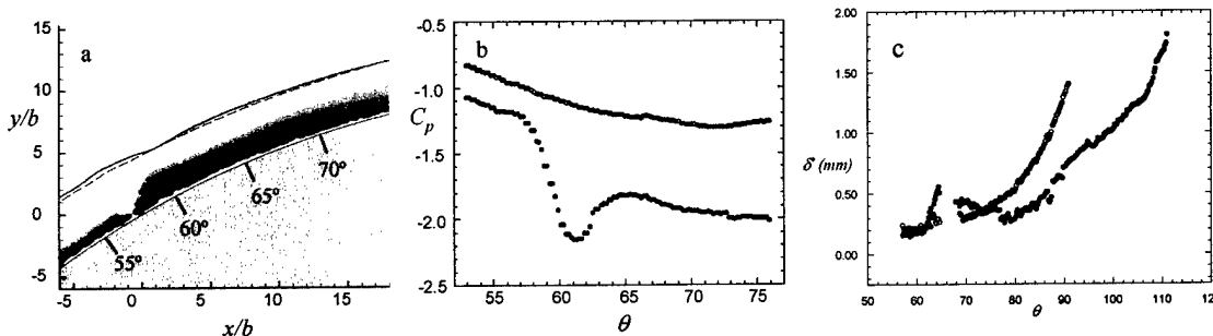
Figure I.2. (a) Vorticity in interaction domain superimposed with streamlines having the same stream function value: baseline (----) and actuated (—); The pressure coefficient along the streamlines (b) and the boundary layer displacement thickness (c): baseline ( \circ ), actuated ( \bullet ).
