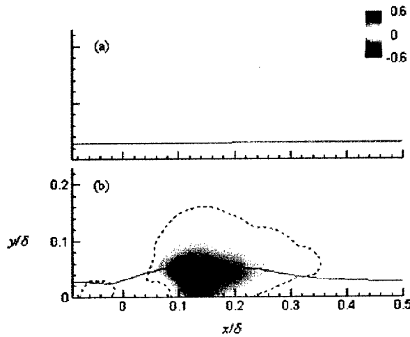
Figure IV.12. Normalized pressure field with \hat{\psi} = 0.01 superimposed: (a) baseline, (b) actuated. Dashed line indicates least significant contour of negative pressure, \bar{p} = -0.025\left(\frac{1}{2}\rho U_\infty^2\right)
