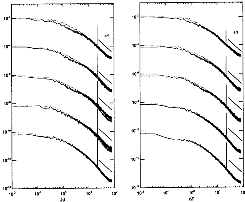
Figure IV.18. u power spectra (baseline in gray) Left: x/\delta = 1.3 , y/\delta = 0.032, 0.065, 0.097, 0.16, and 0.26 (top to bottom). ( y^+ = 30, 60, 90, 145, and 240 ) Right: x/\delta = 1.9 , y/\delta = 0.032, 0.065, 0.13, 0.26, and 0.52 (top to bottom). ( y^+ = 30, 60, 120, 240, and 470 ). Successive locations displaced by two decades.
