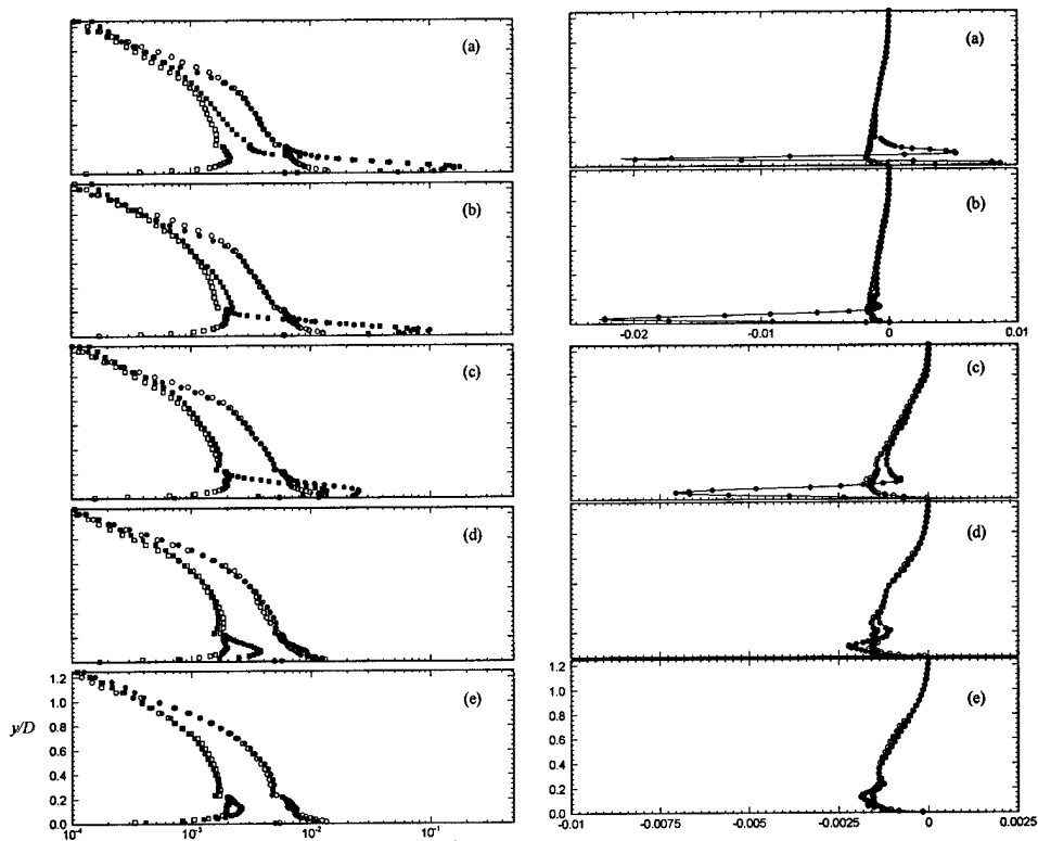
Figure IV.9. Distribution of Left \overline{u'u'}/U_\infty^2 , and \overline{v'v'}/U_\infty^2 : baseline: (○), (□); and actuated: (●), (■) and Right: \overline{u'v'}/U_\infty^2 : baseline (○), actuated (●). x/\delta = 0.13 (a), 0.25 (b), 0.5 (c), 1.0 (d), and 1.5 (e). Note the change in ordinate.
