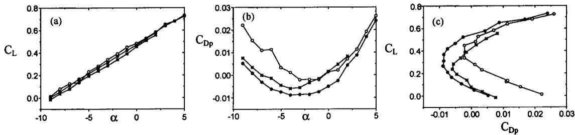
Figure II.10. Lift coefficient (a) and pressure drag coefficient (b) as a function of \alpha , and the pressure drag polar (c). ( \circ ) baseline, ( \bullet ) upstream jet is on and ( * ) downstream jet is on.
