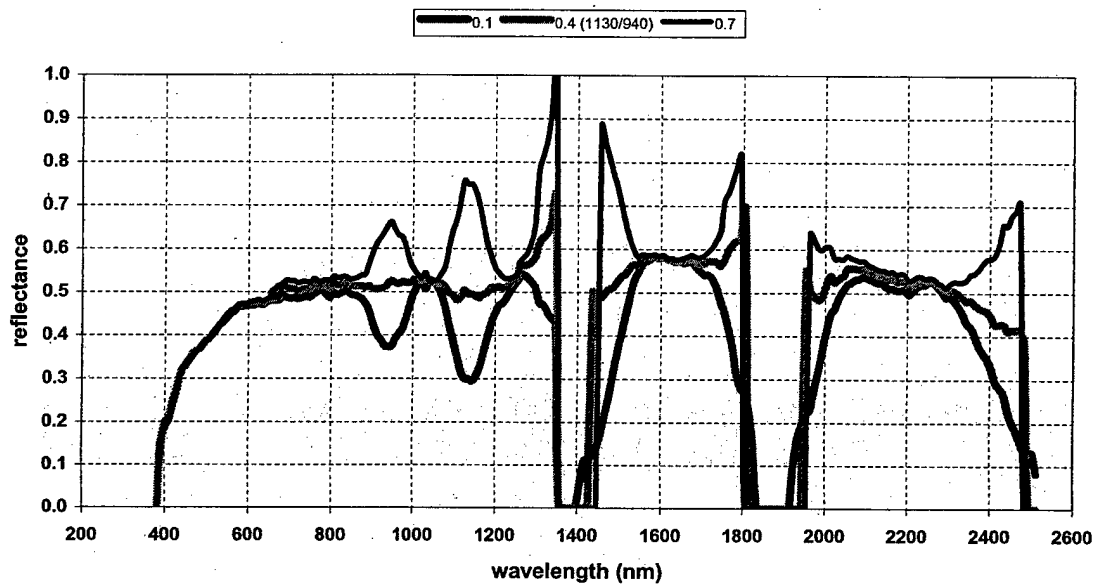
Fig. 5. Building reflectance spectra retrieved by FLAASH using three very different water vapor column amounts.
