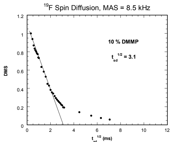
Figure 3. Fluorine-19 Spin Diffusion Return to Equilibrium for 10 wt% DMMP
