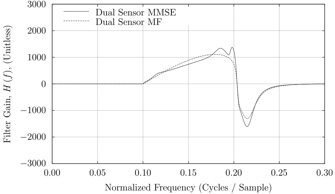
Figure 33. Vertical Two-sensor Filter Component
