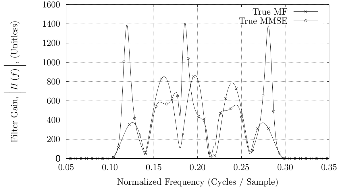
Figure 25. Filters appropriate in a multipath environment
