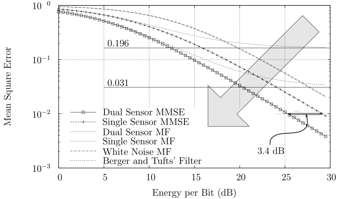
Figure 34. Dual Sensor Mean Square Error. The lines for the two MMSE filters are predictions, and the points are arrived at via simulation. All other lines are arrived at via simulation.
