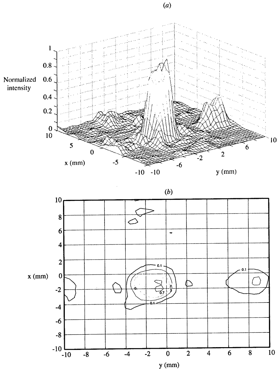
Figure 9. Exosimetry results of the normalized intensity for off-axis focusing with the focal point aimed at -2, -0.7, 30 mm plotted as (a) a mesh or (b) a contour with levels indicated at 90, 70, 50, 30, 10%. These results indicate acceptable grating lobes of less than -7.0 dB.
