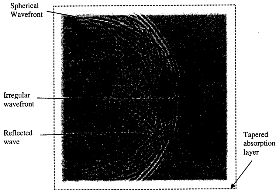
Figure 10: a 2D Gray scaled image showing a background layer of the absorption distribution through middle slice of the 3D prostate model, the tapered absorption boundary layer is shown at the edges with sharp white color. A black dotted line is surrounding the image to distinguish the absorption layer. A spherically propagated wave is shown on top of this background image showing the wave propagation from left to right through the 3D prostate model. The scattered wave is shown following the three cycles wave that has a frequency of 1.2 MHz. Due to sound speed and density changes through this model the wave front is shown with irregular shape while propagating through the urethra area.
