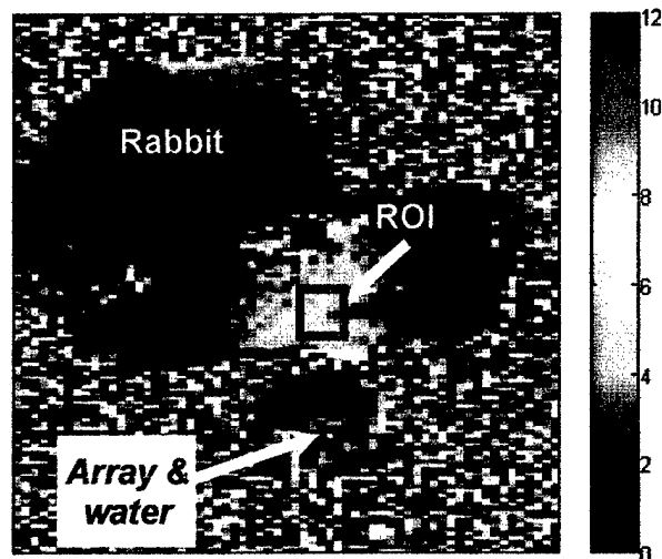
Figure 20. The temperature map (temperature change indicated by the color bar on the right of the figure in ^{\circ}\text{C} ) of the axial view of the MRI-guided in vivo ultrasound hyperthermia experiments setup.
