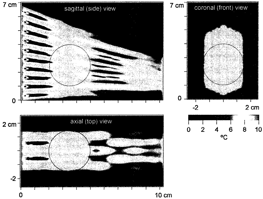
Figure 11. The temperature rise due to heating from all the elements.
