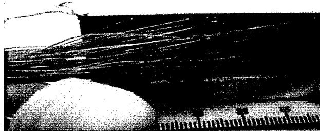
Figure 15: The soldering of sixty miniature coaxial cables is shown; each element of the array was soldered to the core of the coaxial cable. Four points were connected to different points of the conductive matching layer to be soldered to the shield connection of each coaxial cable.
