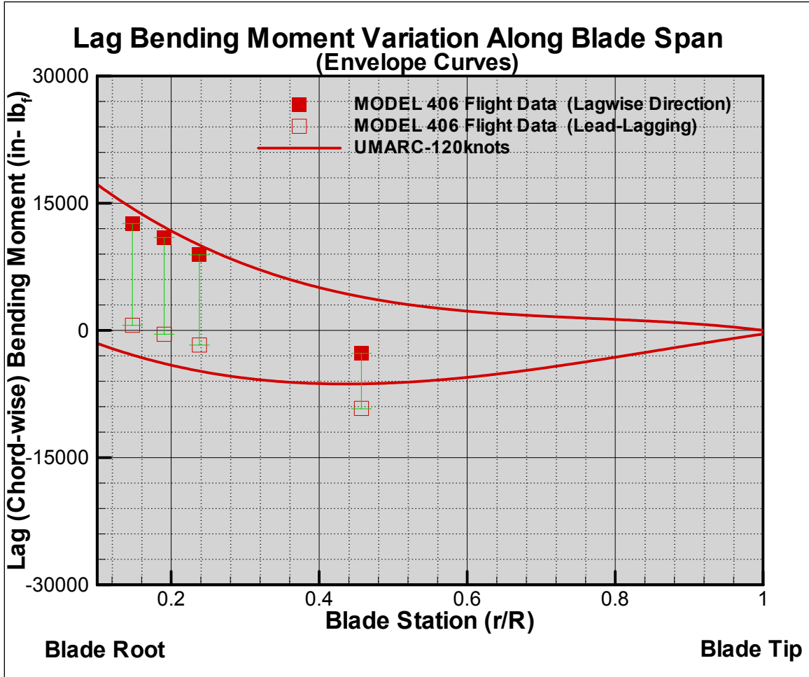
Figure 5. Correlation of lag bending moments along blade span ( \mu = 0.28 ).
