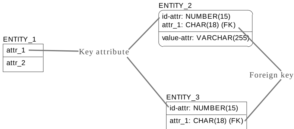
Figure A-3. IDEF1X Display of Attributes
