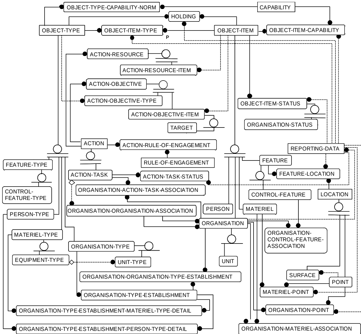
Figure 20. Principal LC2IEDM Entity Structure for WARSIM Unit Data
