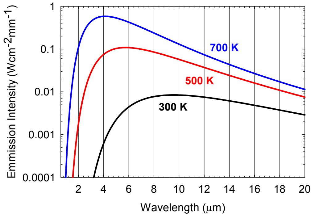
Fig. 12 – Calculated blackbody curves for 300 K, 500 K, and 700 K
