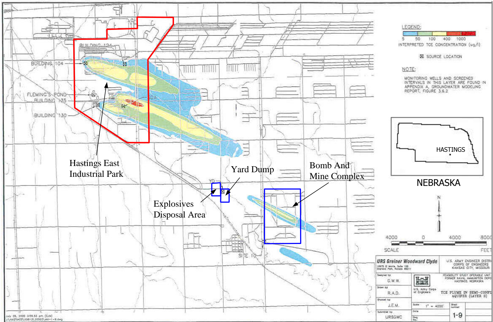
Figure 3-3. Site Location Map With TCE Distribution in Upper Semi-Confined Aquifer, Former Blaine Naval Ammunition Depot
