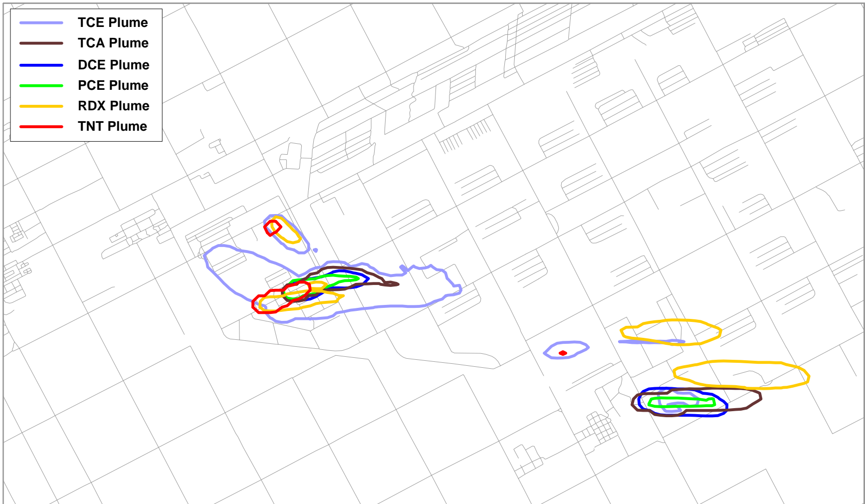
Figure 3-7. Commingled Plumes in Model Layer 1, 8/31/2002, Blaine
