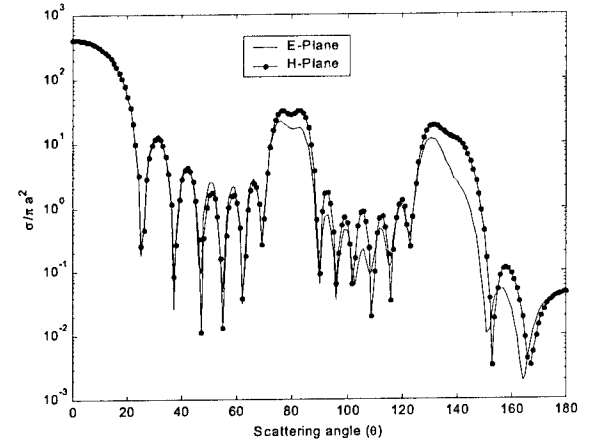
Fig. 5: Normalized bistatic cross-section patterns for eight identical dielectric spheres each covered with a dielectric layer with ka=2.0 , kb=2.5 , kd=7.0 , \alpha=0 , \epsilon_{lr}=3.0 , and \epsilon_{llr}=2.0 .
