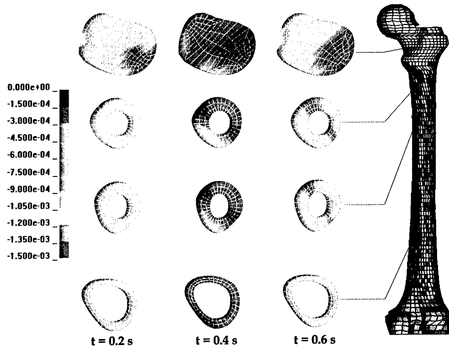
Figure 10: FEM simulation results showing compressive strain (i.e., 3 rd principal strain) of bone cross sections during normal gait for subject S1P6T2 when (a) joint torque and force boundary conditions and (b) muscle force and joint force boundary conditions are imposed.
