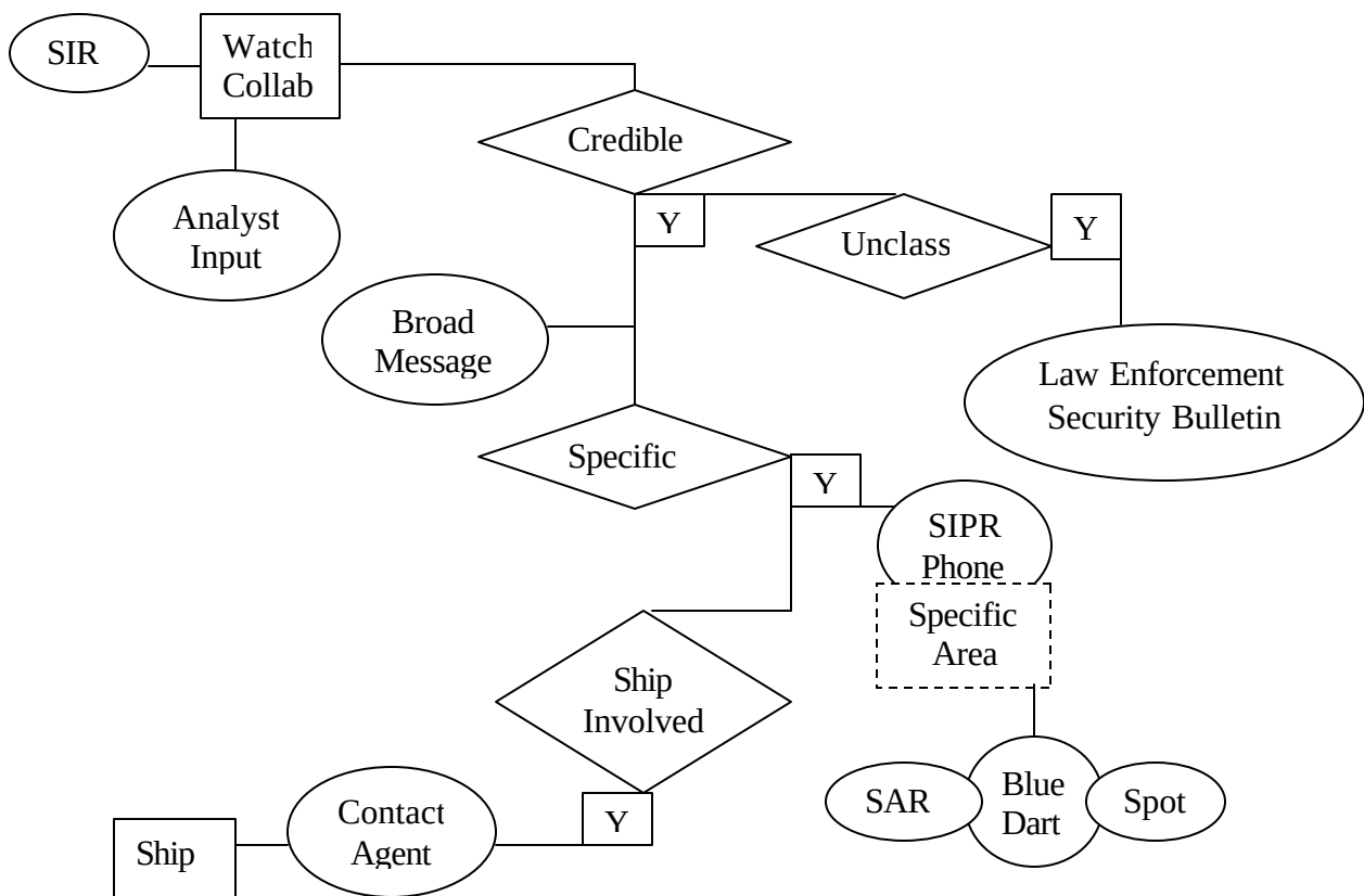
Time-Sensitive Information Flow
