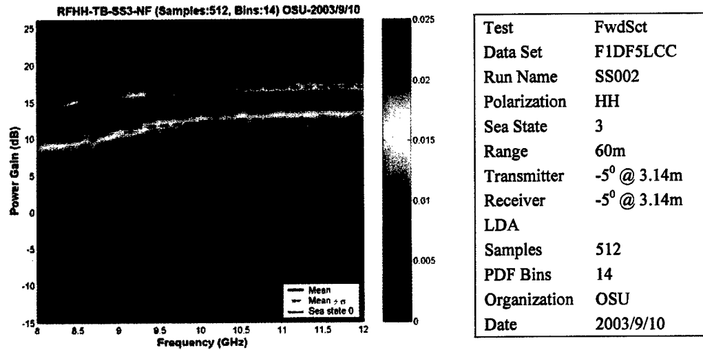
Figure 4.3: Backscatter probability density function (PDF) for sea state 3, non-floating cylinder, horizontal polarization.
