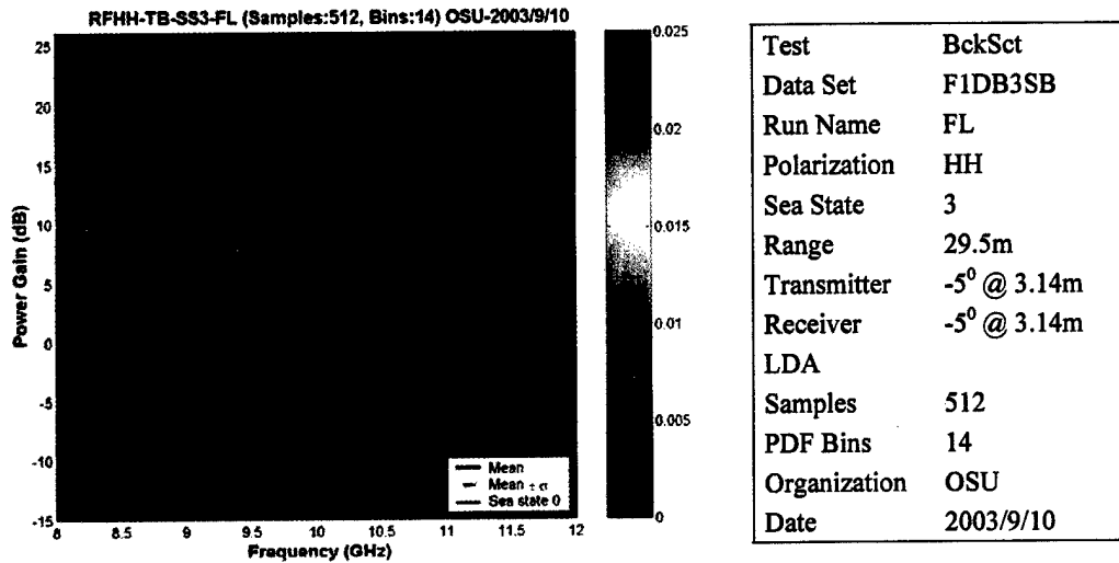
Figure 4.2: Backscatter probability density function (PDF) for sea state 3, floating cylinder, horizontal polarization.
