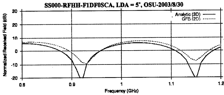
(a) Receiver at position A (height = 0.75m).
