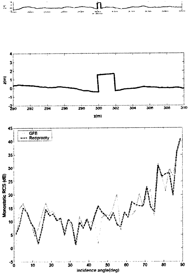
Figure 5.4: Backscatter from a 2m x 1m block on a rough sea surface (sea state 3) computed using GFB and hybrid method using reciprocity. Frequency is 1 GHz, horizontal polarization.
