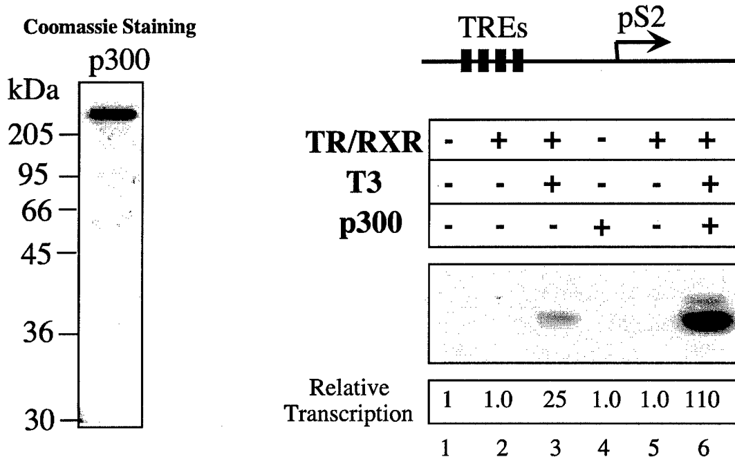
Figure 3. Purified recombinant p300 is functionally active in vitro. (A) Coomassie blue staining of recombinant p300 purified from SF9 cells using Ni-NTA agarose beads. (B) The purified p300 stimulated T3-dependent activation by TR/RXR in a cell-free transcription system.
