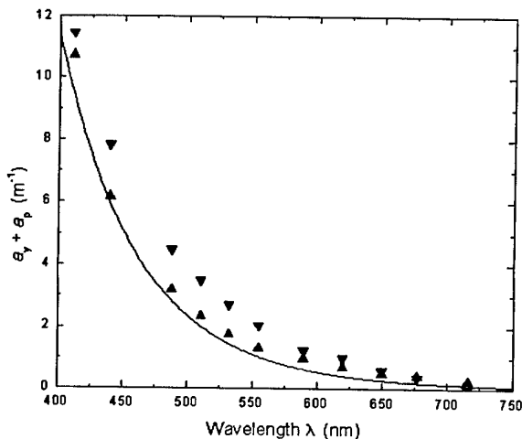
Fig. 9. Downward-pointing triangles \alpha(\lambda) (without a_w ) for the waters of Pearl River, Miss. Upward-pointing triangles, the sum of \alpha_y(\lambda) measured with a 0.045- \mu\text{m} pore filter at the intake of the ac9 meter plus \alpha_p(\lambda) determined from a filter-pad transmission measurement. Solid curve, \alpha(\lambda) obtained from the sequential fit from relation (4).
