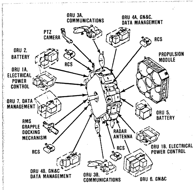
Figure 3: Fully Modular Design and Orbital Replacement Units (ORUs) Enable On-Orbit Maintenance.
