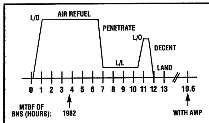
Figure 1. FB-111A Mission Profile Compared to Mean Time Between Failure of Bombing Navigation System.
