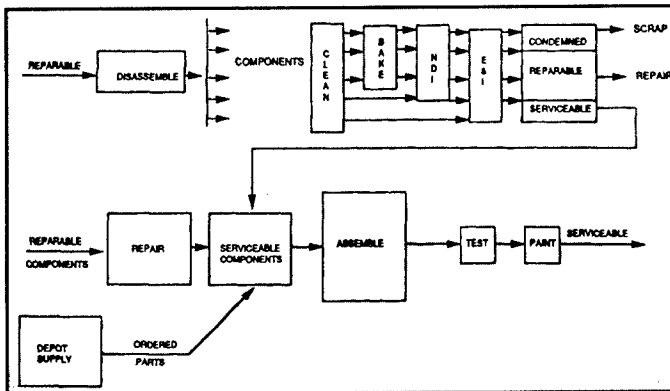
Figure 3. Typical disassembly and repair flows.
