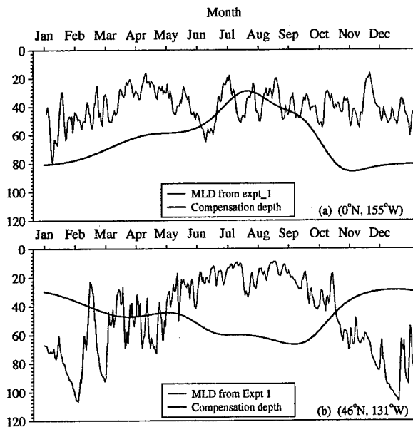
FIG. 7. Compensation depths computed from k_{PAR} for the two mooring locations shown in Fig. 4. Also shown are daily time series of model MLD from experiment 1.
