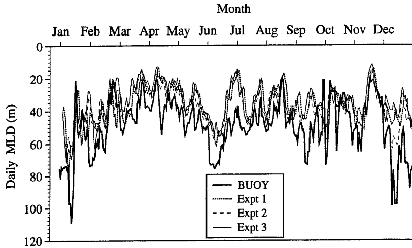
FIG. 6. Daily averaged MLD time series comparisons between values calculated from buoy subsurface temperatures and those from the three NLOM experiments at (0°, 155°W) in 1997. See Fig. 5 for monthly k_{PAR} values at this location.
