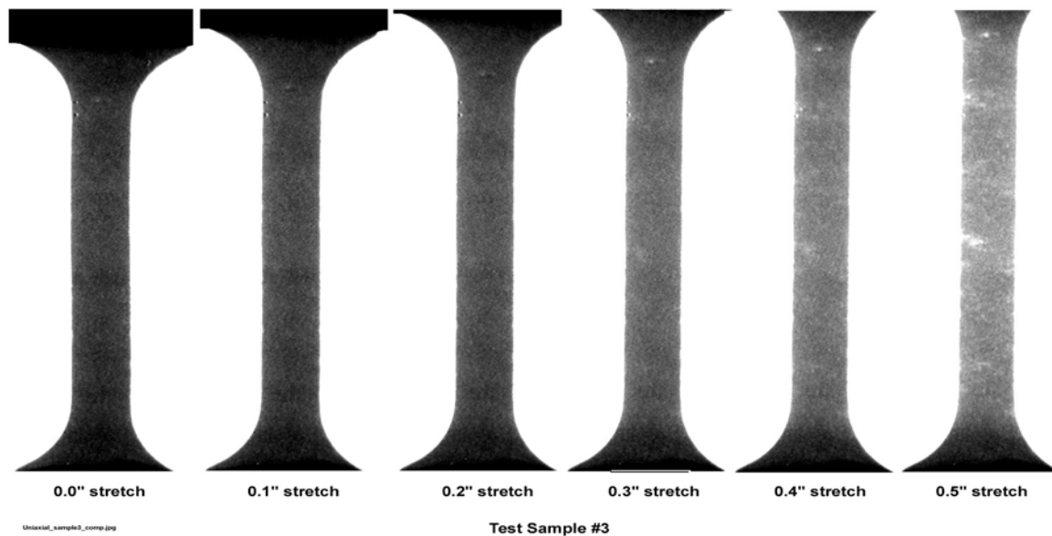
Figure 3. X-Ray Images of Sample 3 at Different Amounts of Stretch
