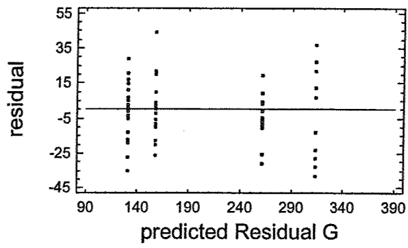
Residual Plot for Residual G
