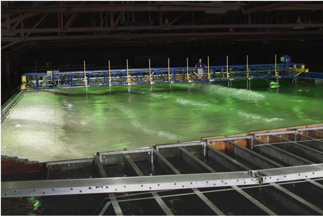
Fig. 1. An experiment in progress at the LSTF
