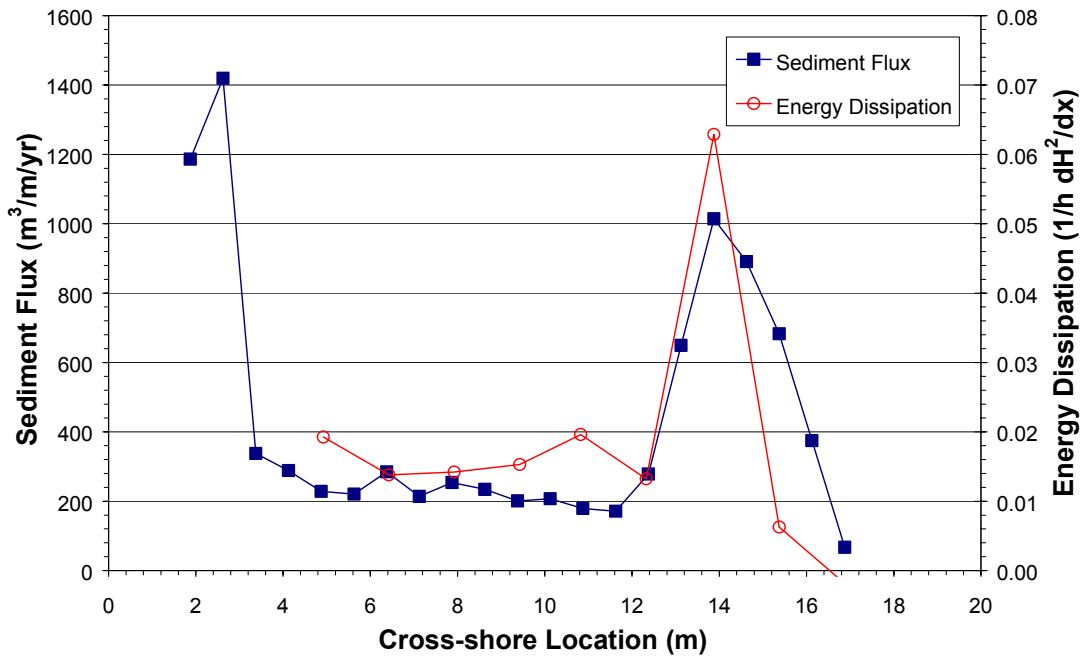
Fig. 6. Sediment flux and energy dissipation for plunging waves
