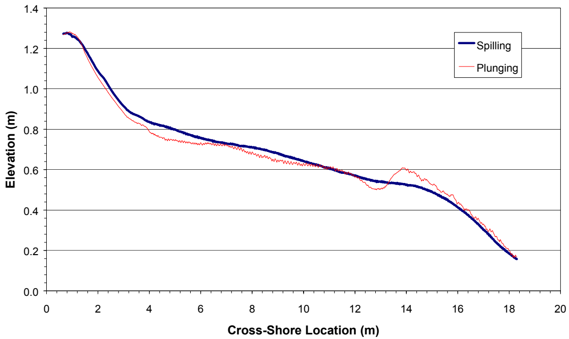
Fig 3. Equilibrium profiles formed by spilling and plunging breakers
