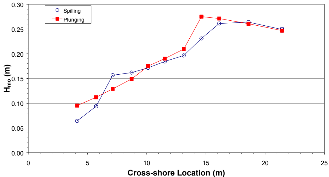
Fig 2. Wave transformation of spilling and plunging breakers
