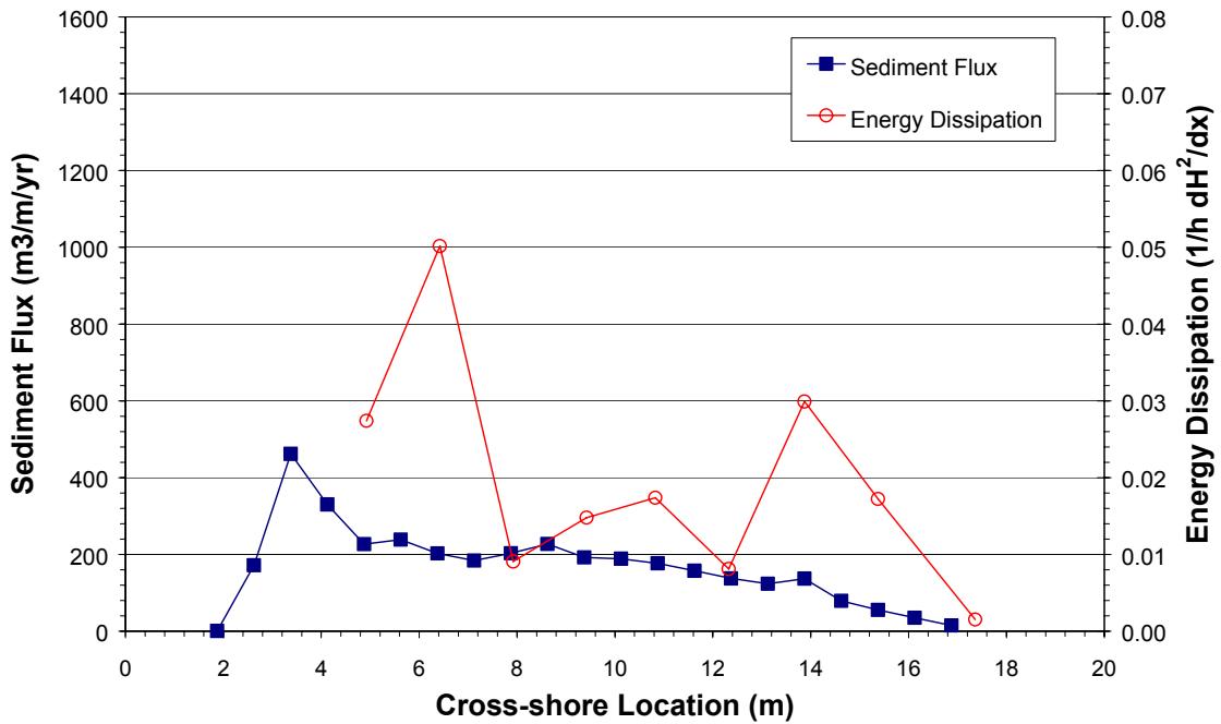
Fig. 7. Sediment flux and energy dissipation for spilling waves
