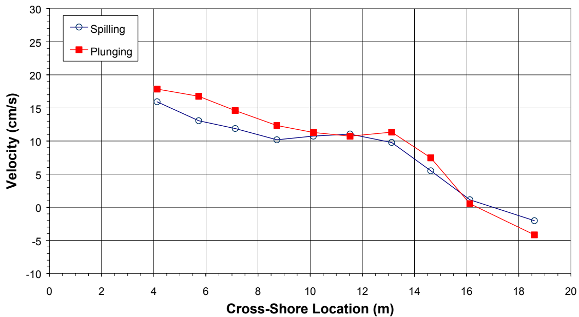
Fig. 4 Distribution of longshore currents produced by spilling and plunging waves
