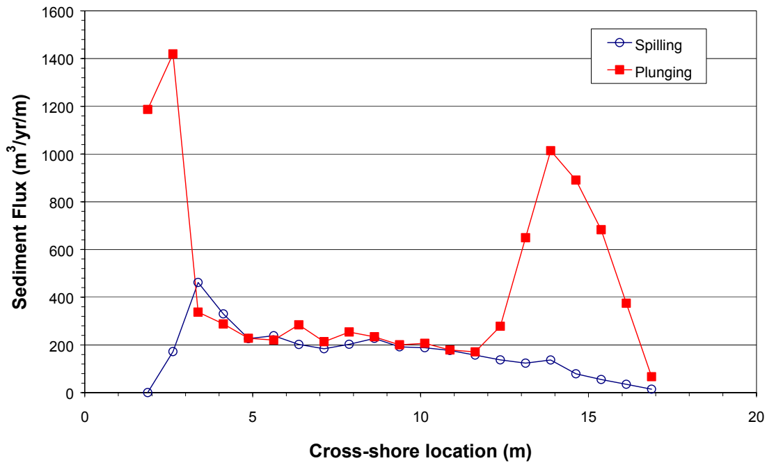
Fig. 5. Sediment flux distribution of spilling and plunging waves
