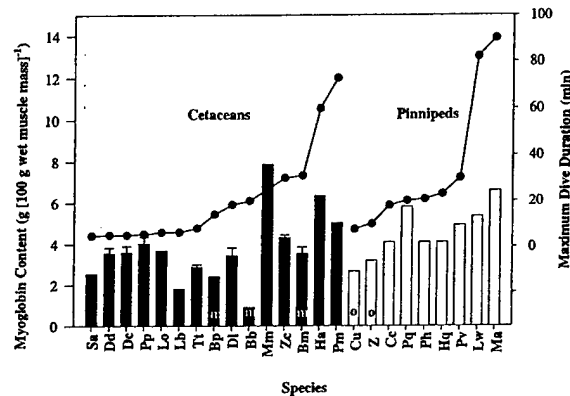
Fig. 4. Muscle myoglobin content (bars) and maximum dive duration (—●—) for cetaceans (black bars) and pinnipeds (white bars). Individual species are ordered in order of increasing dive duration. 'm' denotes mysticetes and 'o' denotes otariids. Initials denote genus and species. Note that our calculations show that in pinnipeds, myoglobin concentration correlates with maximum dive duration according to the relationship, \text{dive duration} = 18.7 [\text{Mb}] - 51.4 ( r^2 = 0.58 , F = 9.82 , P = 0.017 , n = 9 ). The relationship between maximum dive duration and myoglobin content is more variable in cetaceans as described in the text. See Table 1, Table 2, and Table 3 for cetacean references. (Sa, Stenella attenuata ; Dd, Delphinus delphis ; Dc, Delphinus capensis ; Pp, Phocoena phocoena ; Lo, Lagenorhynchus obliquidens ; Lb, Lissodelphis borealis ; Tt, Tursiops truncatus ; Bp, Balaenoptera physalus ; Dl, Delphinapterus leucas ; Bb, Balaenoptera borealis ; Mm, Monodon monoceros ; Zc, Ziphius cavirostris ; Bm, Balaena mysticetus ; Ha, Hyperoodon ampullatus ; Pm, Physeter macrocephalus ). Pinniped references Otariids: Cu, Callorhinus ursinus : [Mb] (Lenfant et al., 1970; Castellini and Somero, 1981), Dive (Gentry et al., 1986); Z, Zalophus californianus : [Mb] (Castellini and Somero, 1981), Dive (Feldkamp et al., 1989). Phocids: Cc, Cystophora cristata : [Mb] and Dive (Scholander, 1940); Pg, Phoca groenlandica : [Mb] and Dive (George et al., 1971); Ph, Phoca hispida : [Mb] (Lydersen et al., 1992), Dive (Parsons, 1977); Hg, Halichoerus grypus : [Mb] (Scholander, 1940), Dive (Lavigne and Kovacs, 1988); Pv, Phoca vitulina : [Mb] (Lenfant et al., 1970; Castellini and Somero, 1981), Dive (Kooyman et al., 1972); Lw, Leptonychotes weddelli : [Mb] (Ponganis et al., 1993), Dive (Castellini et al., 1993); Ma, Mirounga angustirostris : [Mb] (Thorson, 1993), Dive (Le Boeuf et al., 1993).
