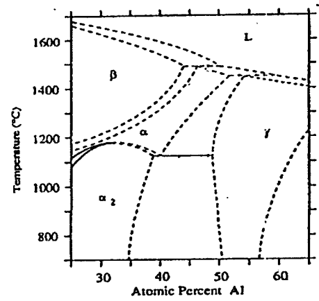
Figure 1 Central portion of TiAl phase diagram.
