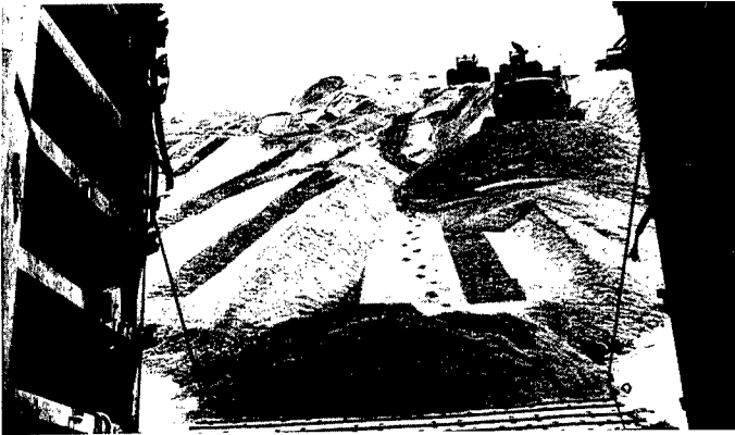
Across the beach delivery. Bulldozers push through the sand to the open doors of a landing ship bringing construction supplies to Tuy Hoa.
