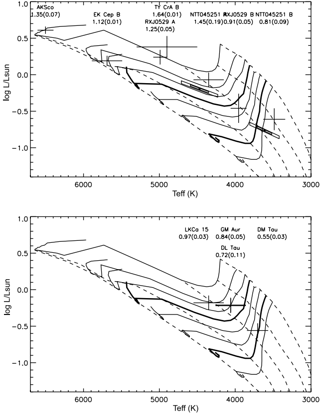
FIG. 22.—Comparison of all PMS stars with accurate empirical mass determinations and M \lesssim 1.6 M_{\odot} with the tracks of BCAH98, \alpha_{\text{in}} = 1.0 . ( Top ) Stars in binary systems. Masses for each of these are indicated at the top of the figure. Mass tracks shown are for 0.6, 0.7, 0.8, 0.9, 1.0, 1.1, 1.2, and 1.4 M_{\odot} . ( Bottom ) Same as above, but for single stars. Note that the uncertainties on the masses of the single stars do not include distance uncertainties, which can amount to \sim 15\% (Simon et al. 2000).
