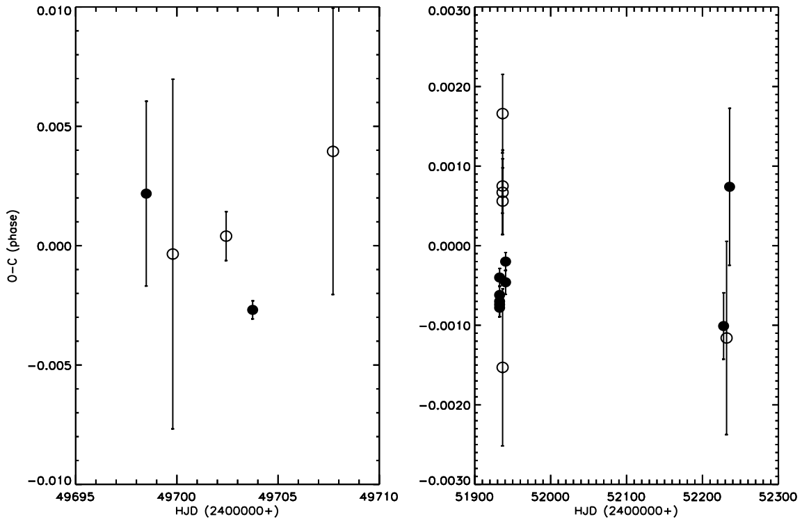
FIG. 8.—The O-C phase residuals of the eclipse timings of V1174 Ori are shown based on a best-fit period of 2.634727 days. Filled circles represent primary eclipses, open circles represent secondary eclipses. See Table 5.
