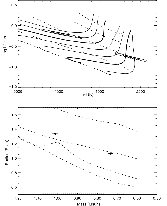
FIG. 20.—Montalbán et al. (2004) tracks with MLT convection ( \alpha_{\text{in}} = 1.0 , \tau_{\text{ph}} = 3 ) and NextGen atmospheres from Hauschildt et al. (1999). Symbols and lines are as in Fig. 16.
