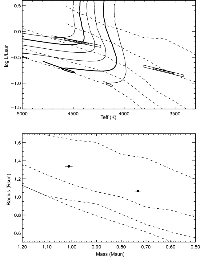
FIG. 19.—SDF00 tracks. Symbols and lines are as in Fig. 16.
