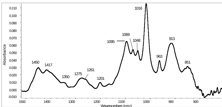
Figure 6.4-4: Unaged Boegel-EPII Solution ( 1500\text{cm}^{-1} - 650\text{cm}^{-1} )
