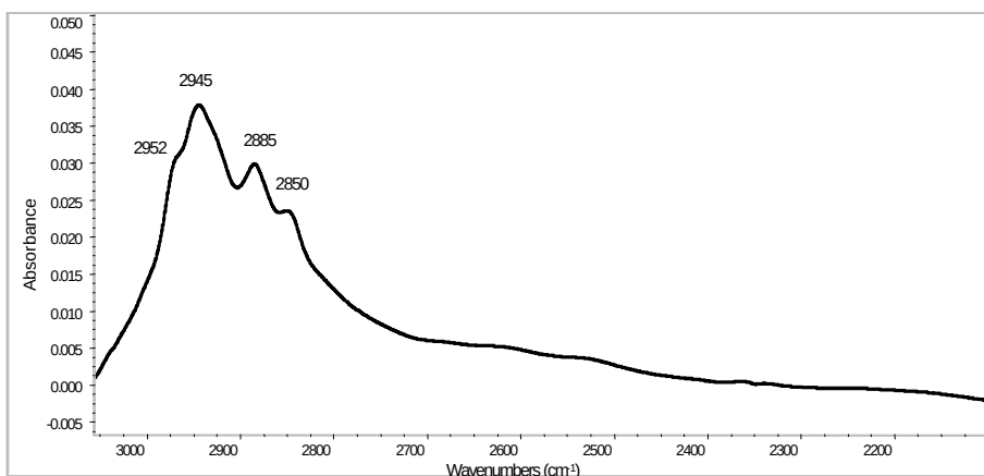
Figure 6.4-5: Boegel-EPII Solution Aged 4 Weeks ( 3100\text{cm}^{-1} - 2100\text{cm}^{-1} )
