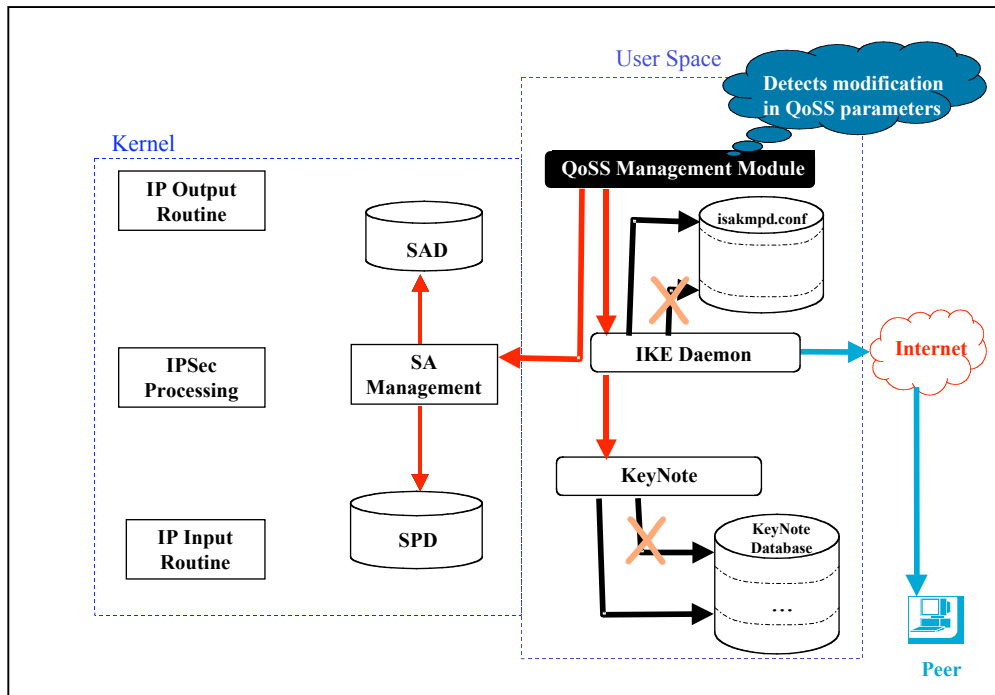
Figure 4: QoSS awareness for IPsec
