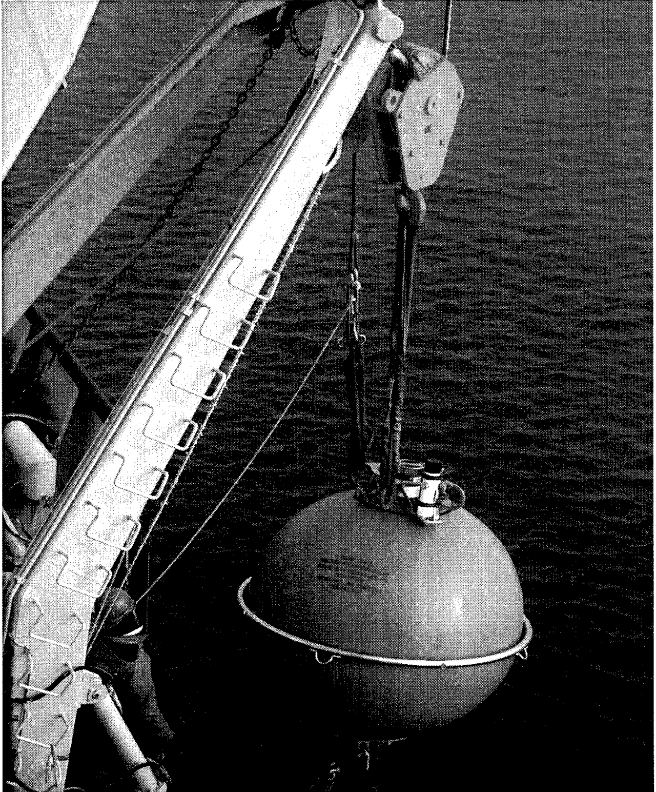
Figure 14. Sling detail: sphere deployment
