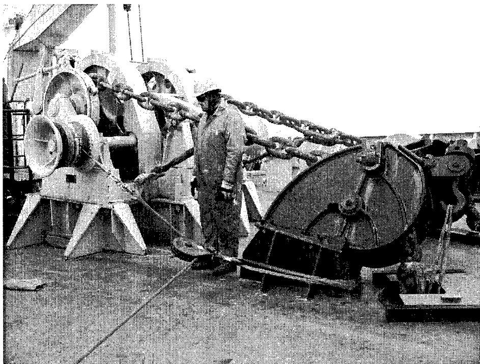
Figure 9. Fair lead block and stopper line
