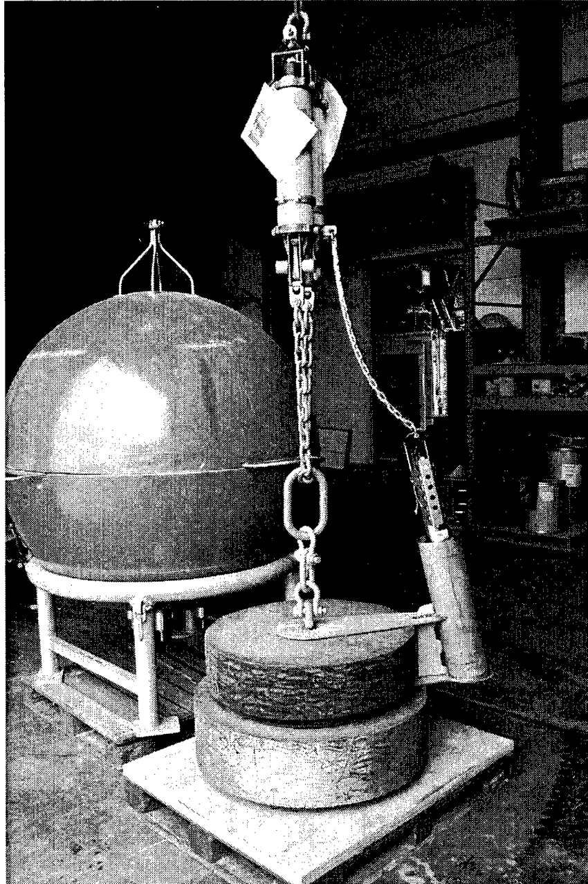
Figure 12. BGFE mooring anchor, SeaCat recorders and dual release package
