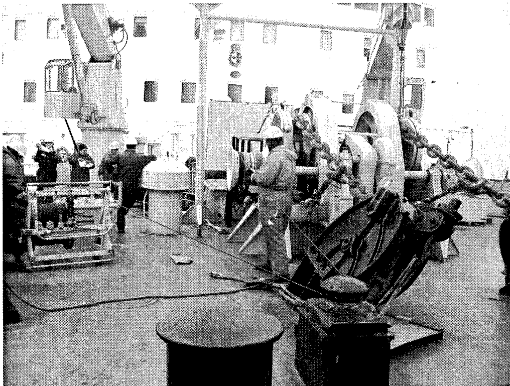
Figure 11. Wire fairlead windlass capstan to tension cart
