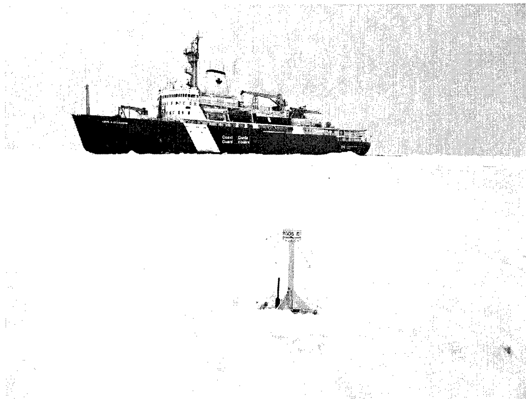
Figure 20. BGFE ice beacon deployed from CCGS Louis S. St. Laurent in summer 2003.
