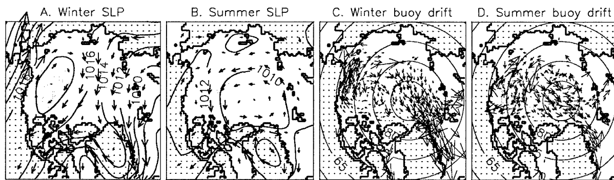
Fig. 2. 1979–1997 winter (A) and summer (B) averaged sea level pressure and geostrophic wind. Seasonal IABP buoy drift is shown in C and D. In winter, the buoy drifts coincide with the anticyclonic wind motion, which generates (by Ekman pumping) a negative salinity anomaly in the BG so that the ocean accumulates potential energy. In summer, this energy supports the anticyclonic geostrophic circulation (Fig. 1D), and drives the buoy drifts against the predominantly cyclonic winds.
