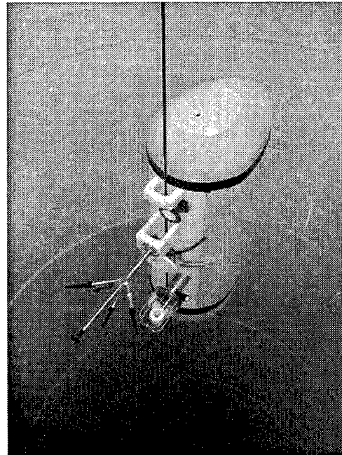
Figure 15. McLane Moored Profiler
