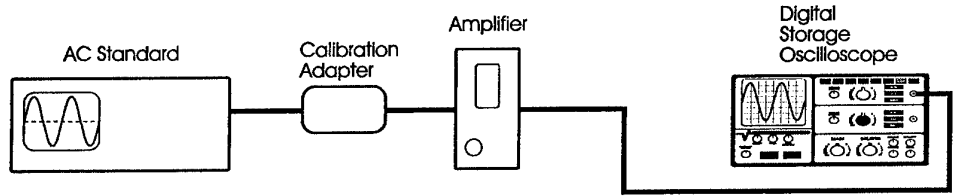
(b) Voltage Calibration Setup
