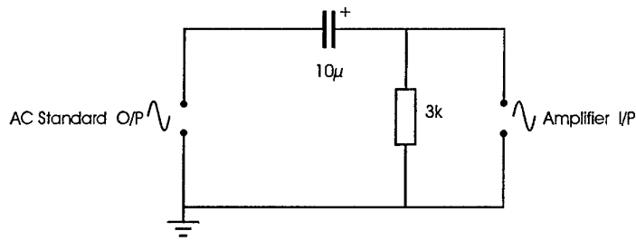
Figure 7: Calibration Adaptor Circuit
