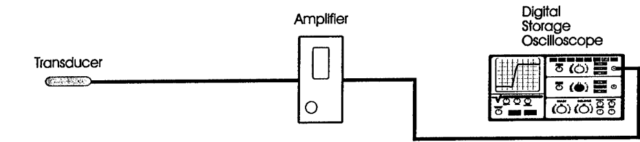
(a) Pressure Calibration Setup
