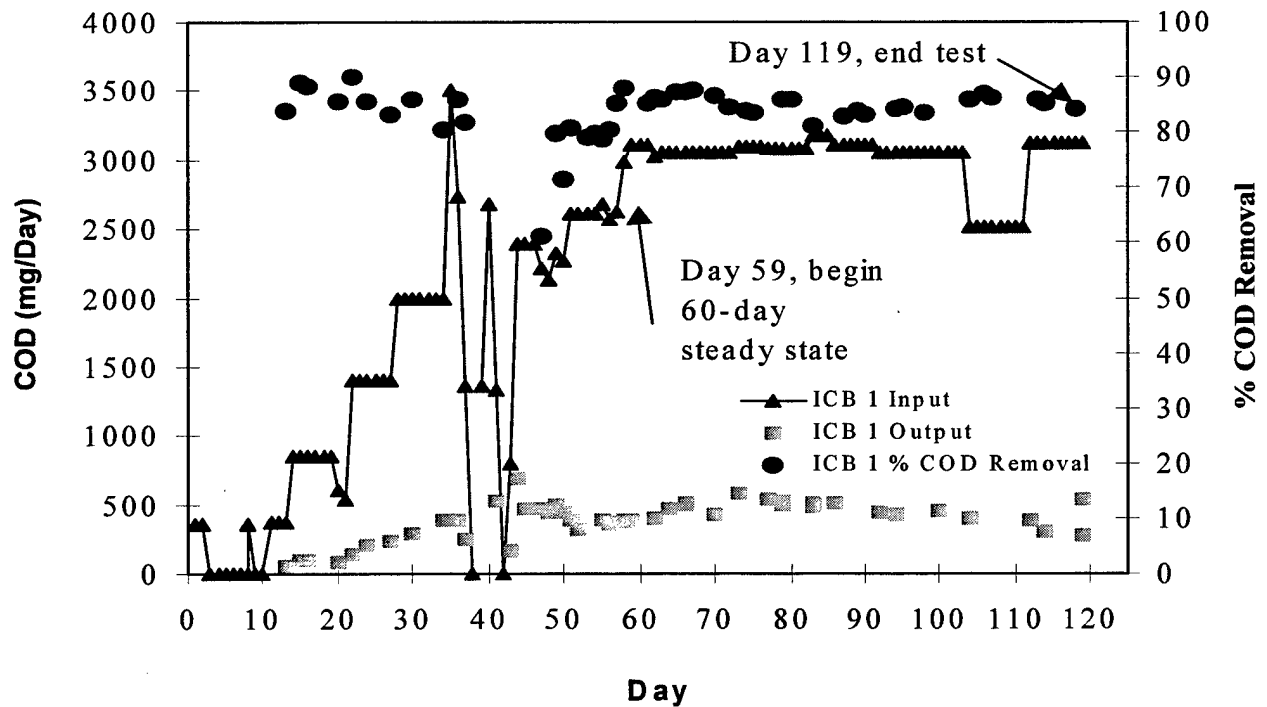
Figure 3. COD Results for ICB 1 (Unfiltered Feed)
