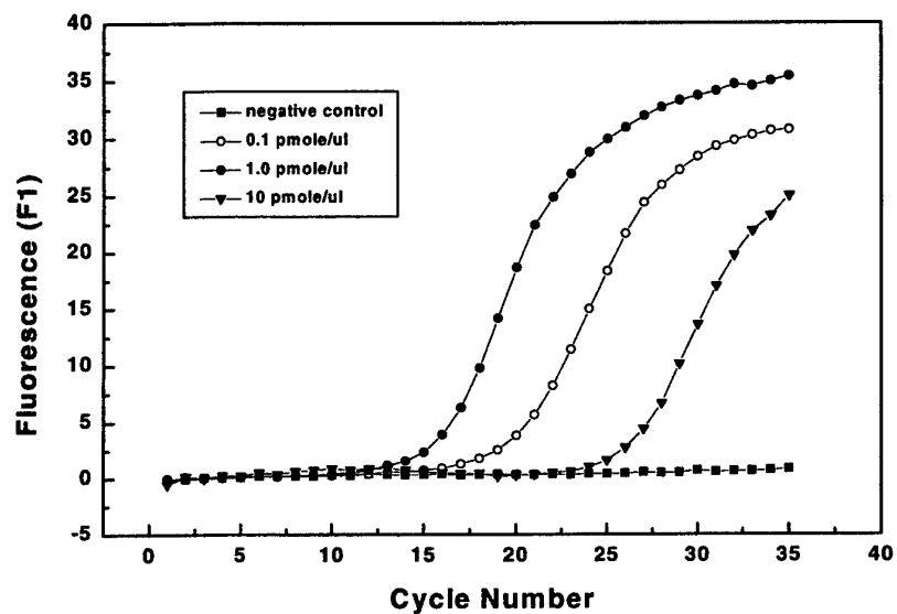
Figure 6: The effect of concentration of the primers BpsF and BpsR on B. pseudomallei PCR.
