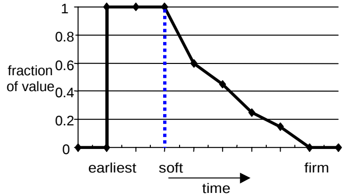
Figure 1: The deadline coefficient graph (non-increasing) shows the variation in the value of a task with various deadlines.
