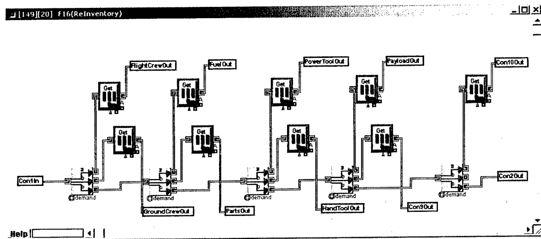
Figure 19: Effects Model Representation of F-16 Inventory Management
