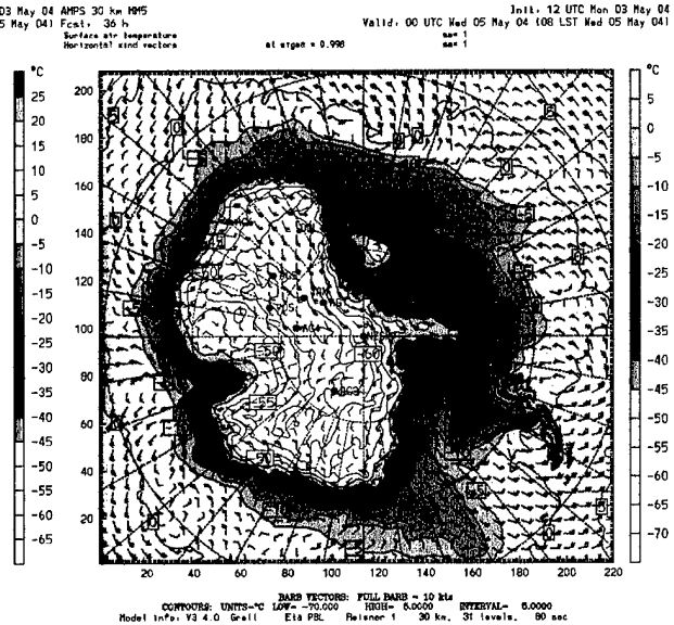
FIG. 20. AMPS 30-km domain, 36-hr surface forecast valid: 00 UTC 05 May 04 (AMPS 2004).
