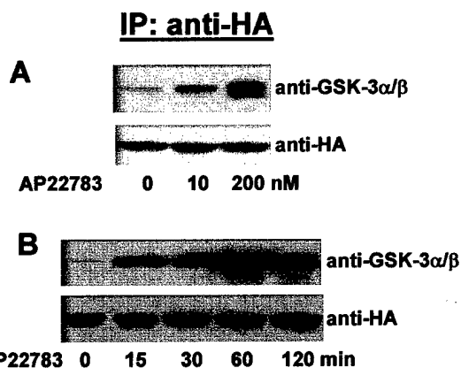
Fig. 4. CID-mediated iAKT activation. LNCaP.iAKT1 cells were serum-starved for 24 h followed by treatment with AP22783 at the doses or for the time period as indicated. The iAKT was immunoprecipitated from cell lysates using anti-HA antibody and incubated with the GSK-3 'crosstide' as a substrate. Phosphorylated GSK-3 crosstides were quantified by SDS-PAGE separation and immunoblotting with a phospho-specific antibody against GSK-3α 21 /β 9 . Anti-HA blot served as loading control.
