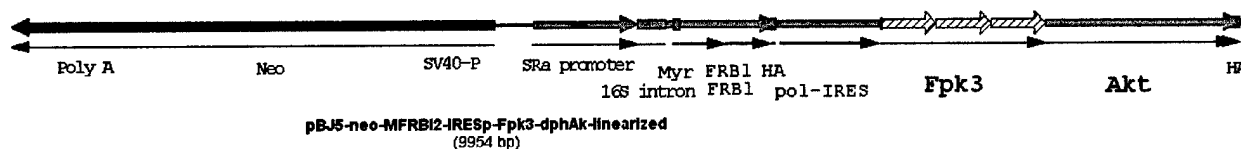
Fig. 1. Schematic representation of the linearized pBJ5-Neo-iAKT plasmid construct
