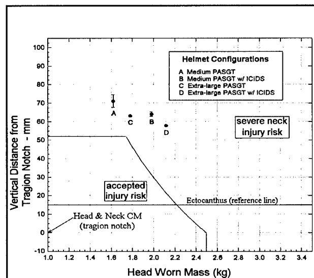
Fig 3. Test helmet mass and vertical (Z-axis) center of mass (tragon notch), plotted against the USAARL-recommended head-supported mass criteria for Army aircrew helmets.
