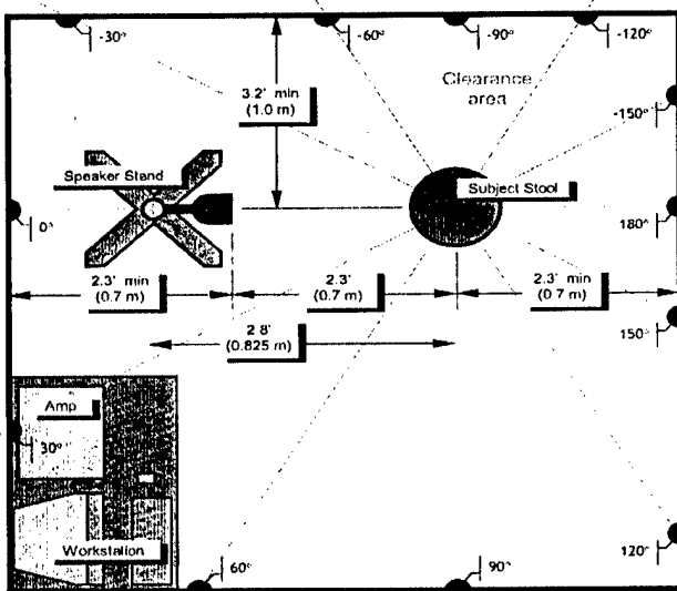
Fig 1. Typical layout of AuSIM3D "HeadZap" measurement system.
