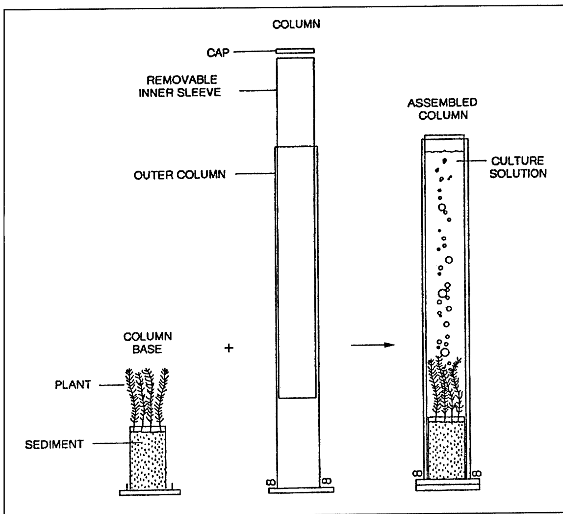
Figure 4. Column assembly
