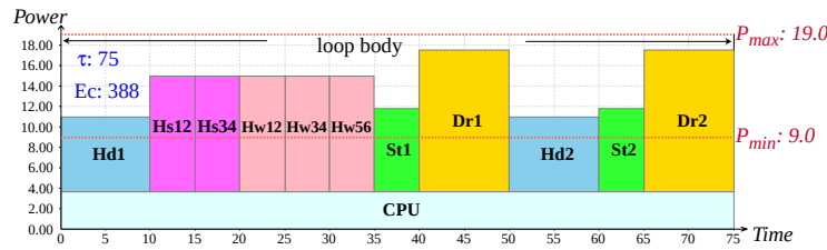
Figure 4.11: The serial schedule for Scenario 3 (lowest power budget).
