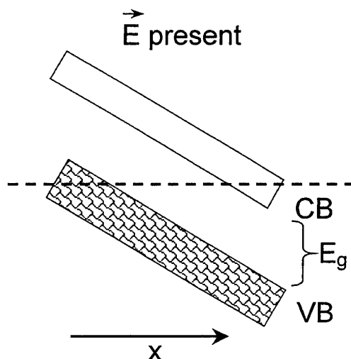
Figure 3-6: Tilted band structure as discussed by Zener Theory
