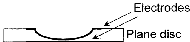
Figure 4-2: The 'Recessed Specimen' Method
