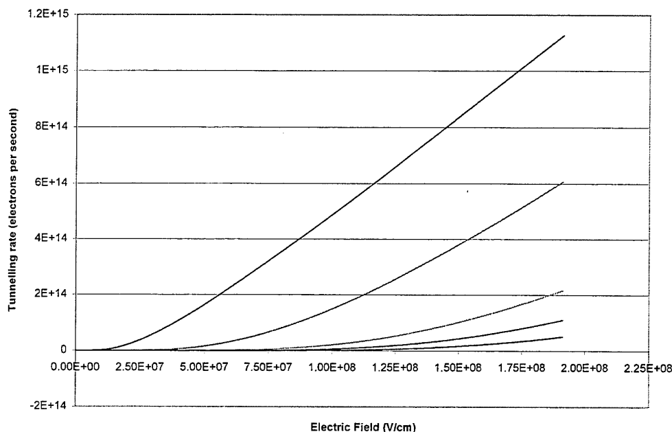
Figure 3-7: Tunnelling Rates as predicted by Zener Theory
