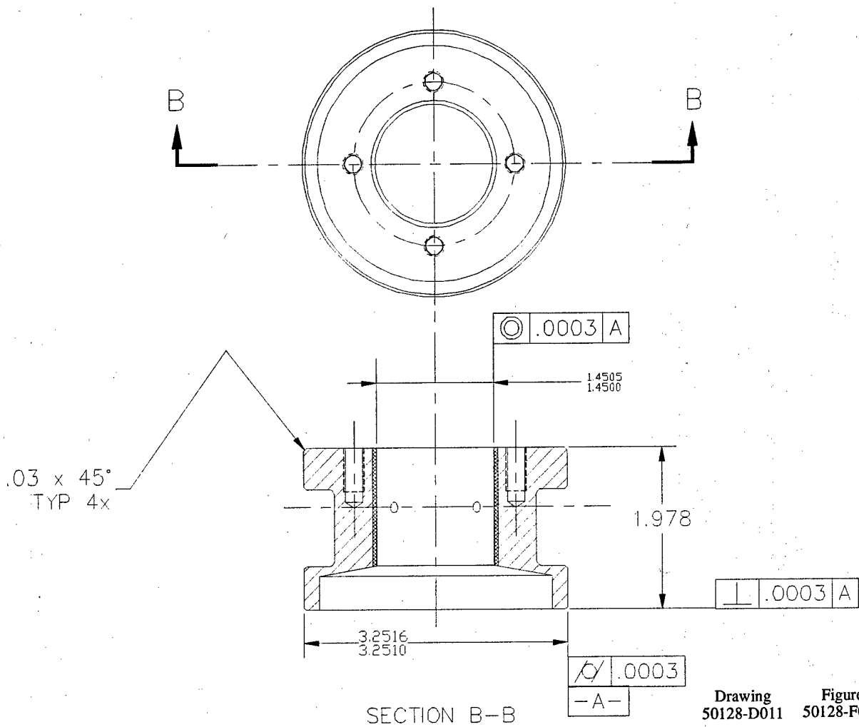
Figure 10. High pressure abradable seal design.
