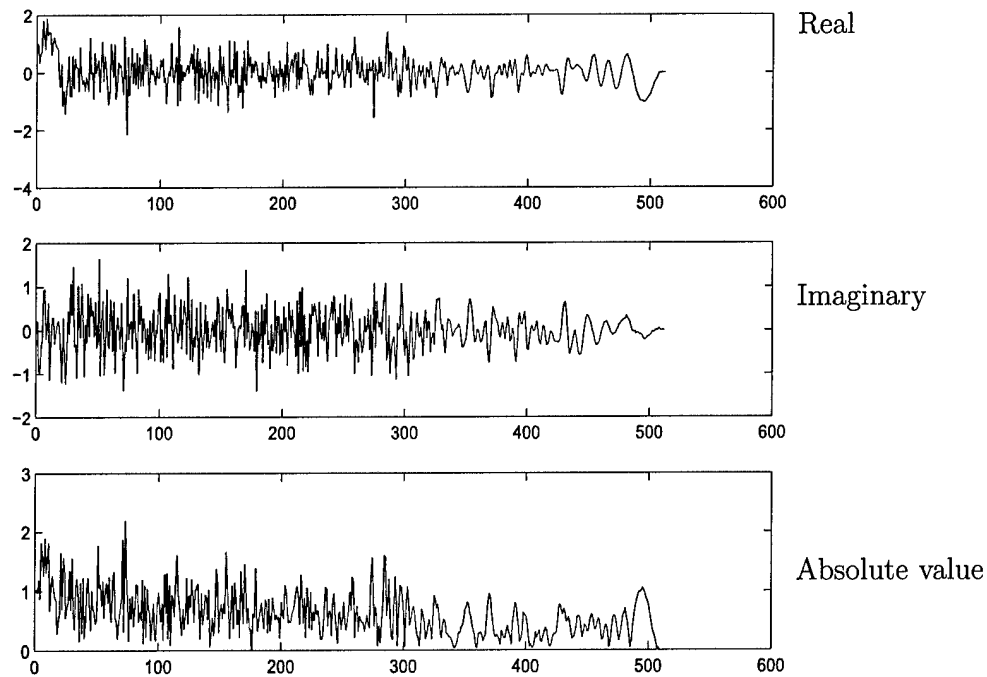
Figure 7.5. Auto-correlation of received, noisy signal with the transmitted chirp.
