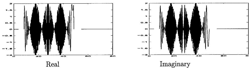
Figure 5.2. Sum of two shifted discrete chirps.
