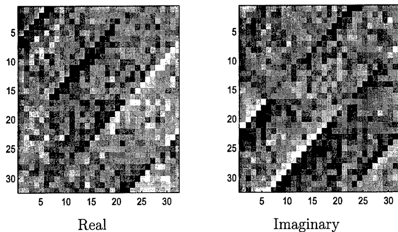
Figure 7.8. Test reflectivity kernel.
